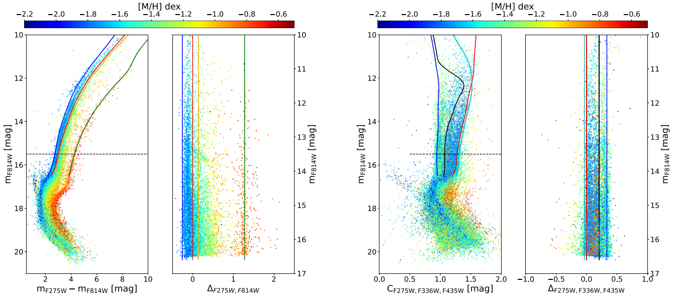
Figure 17. Final fiducial lines. Left: the CMD for all stars; right: the pseudo-CMD. Both are color-coded with [M/H] and show the fiducial lines for the RGB. On the right of each panel is the verticalized CMD, proving that the subsamples do follow these straight lines.
