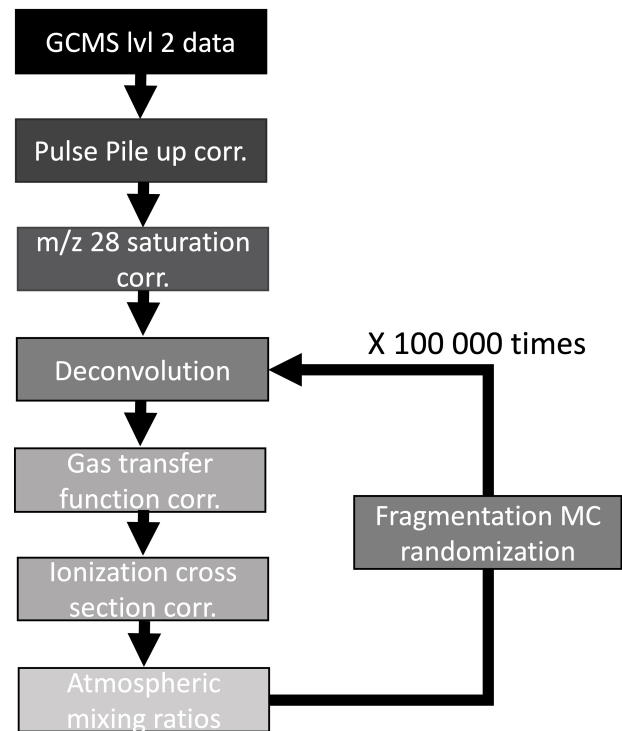
Fig. 3. Schematic representation of the data workflow from retrieved GCMS level 2 data on the PDS to atmospheric mixing ratios.
