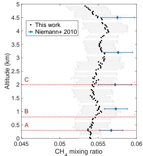
Fig. 6. Close up of the high-resolution profile of methane in the lower troposphere below 5 km. Black dots represent our median retrieved values with their associated error bars. Blue diamonds and bars represent methane mixing ratios reported by Niemann et al. (2010) and their standard deviation, respectively. Red horizontal dashed lines labeled A, B, and C represent the altitude of the boundary layers identified in Charnay & Lebonnois (2012) at 300 m, 800 m, and 2 km, respectively.
