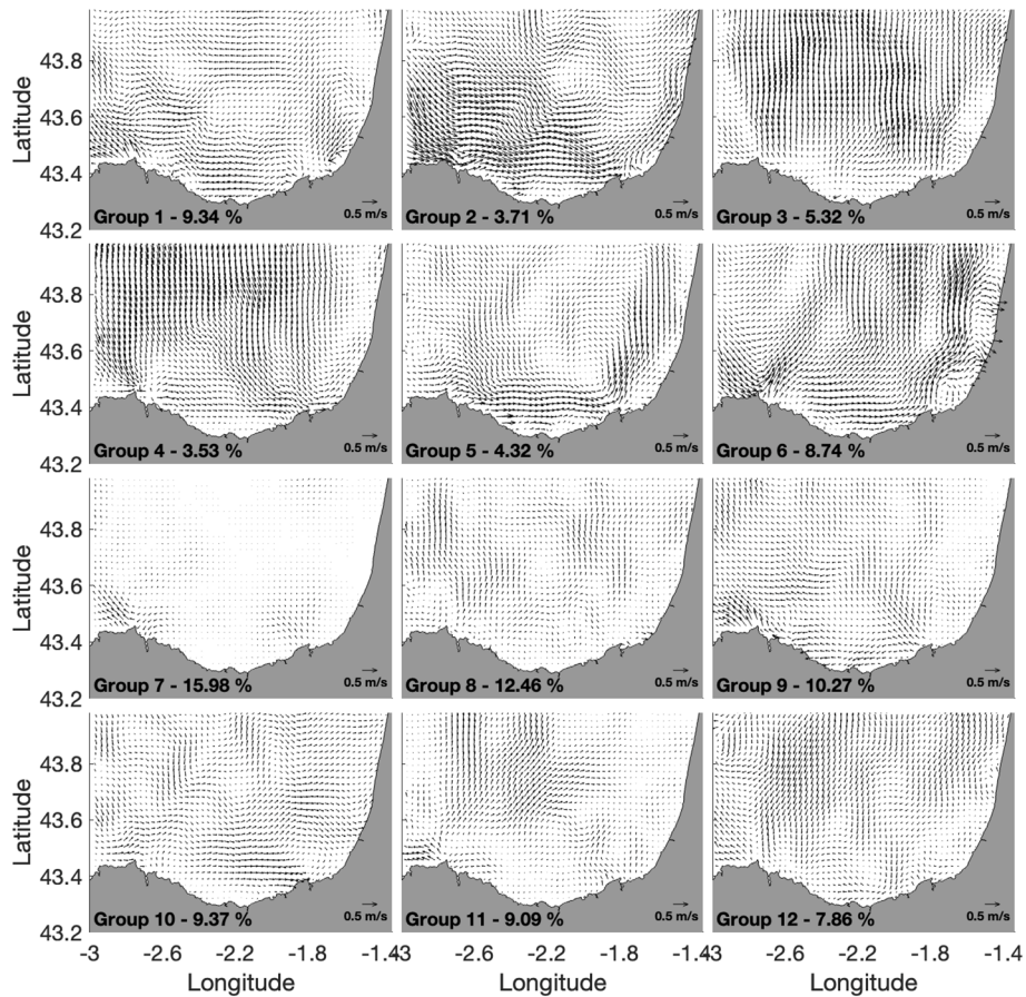
Fig. B2. 4 × 3 lattice of the K-Means algorithm applied to HFR surface currents from January 2020 to December 2022. The percentage of variability explained by each group is given in the title.
