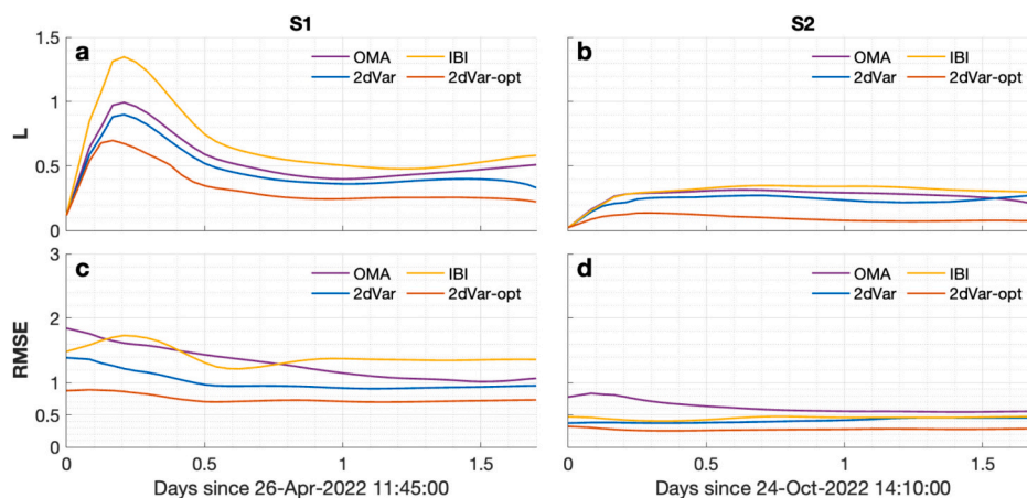
Fig. 4. L index (a, b) and RMSE (c, d) computed for the available fields. Figures related to S1 are given in the left column, while figures related to S2 are given in the right column.
