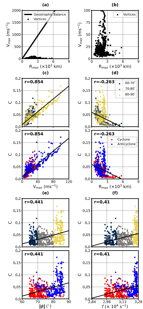
Fig. 10. Vortex dynamics in the polar regions as measured by AMEDA. Vortex edge velocity as a function of vortex radius for all detected vortices (black points), (a) with and (b) without the geostrophic balance condition assuming Ro = 1 (black line). Cyclogeostrophic Rossby number, C , as a function of (c) V_{max} , (d) R_{max} , (e) |\phi| , and (f) f , separated by latitude domain, and with linear fit and Pearson correlation coefficient.
