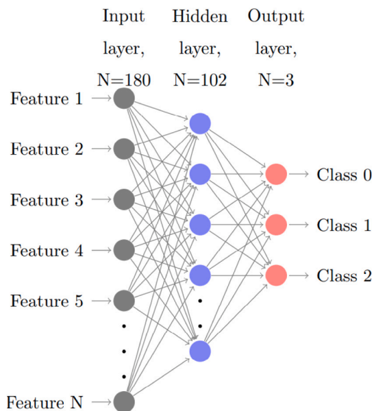
Fig. 4. Schematic of the final neural network architecture. Each input node (grey) represents a feature, i.e. a grid point in the windowed model fields. These are passed to the hidden nodes (blue) then to the output nodes (red) which define the identity of the contents of the window. Bias nodes have been omitted for clarity and arrows represent the neural connections (weights not represented here).
