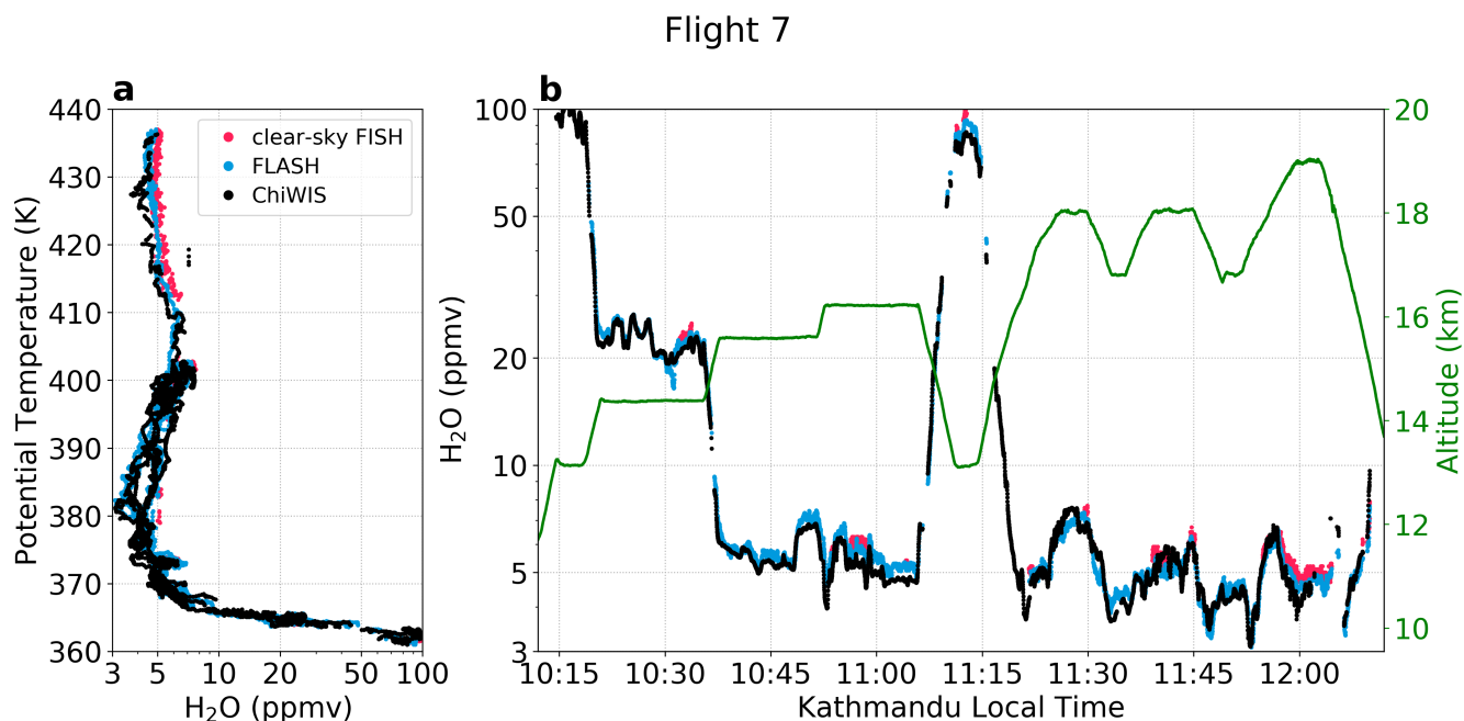
Figure 9. Illustration of multi-instrument agreement: FISH, FLASH, and ChiWIS \text{H}_2\text{O} mixing ratio from Flight 7 of the StratoClim campaign. Agreement is excellent over a range of altitudes and mixing ratios. Figure modified from Singer et al. (2022).
