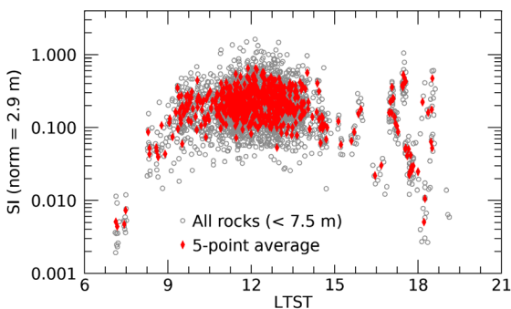
Figure 3. Variations of acoustic scintillation (SI) with local true sol time (LTST), for values normalized at a distance x = 2.9 m.
