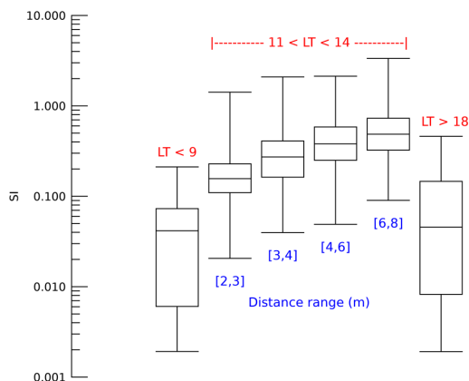
Figure 2. Variations of acoustic scintillation (SI) with local true sol time (LTST) and distance to the target
