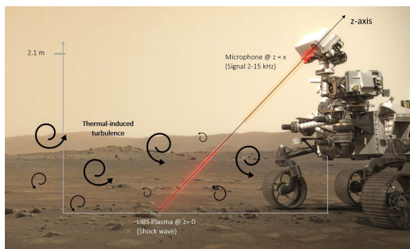
Figure 1. Geometry of the SuperCam microphone recordings of the laser-induced-acoustic signal, where the propagation path (2–8 m) along the z-axis goes through the thermal turbulence generated in the atmospheric surface layer of Mars.
