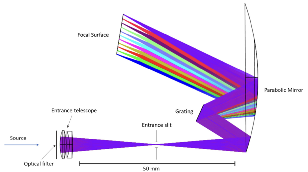
Figure A1. Optical layout of the Uvsq-Sat NG NIR spectrometer (UNIS). UNIS is a miniaturized spectrometer with an aperture of 15 mm, a spectral range from 1100 to 2000 nm, a spectral resolution of 7 nm, and a field of view of 0.15°.
