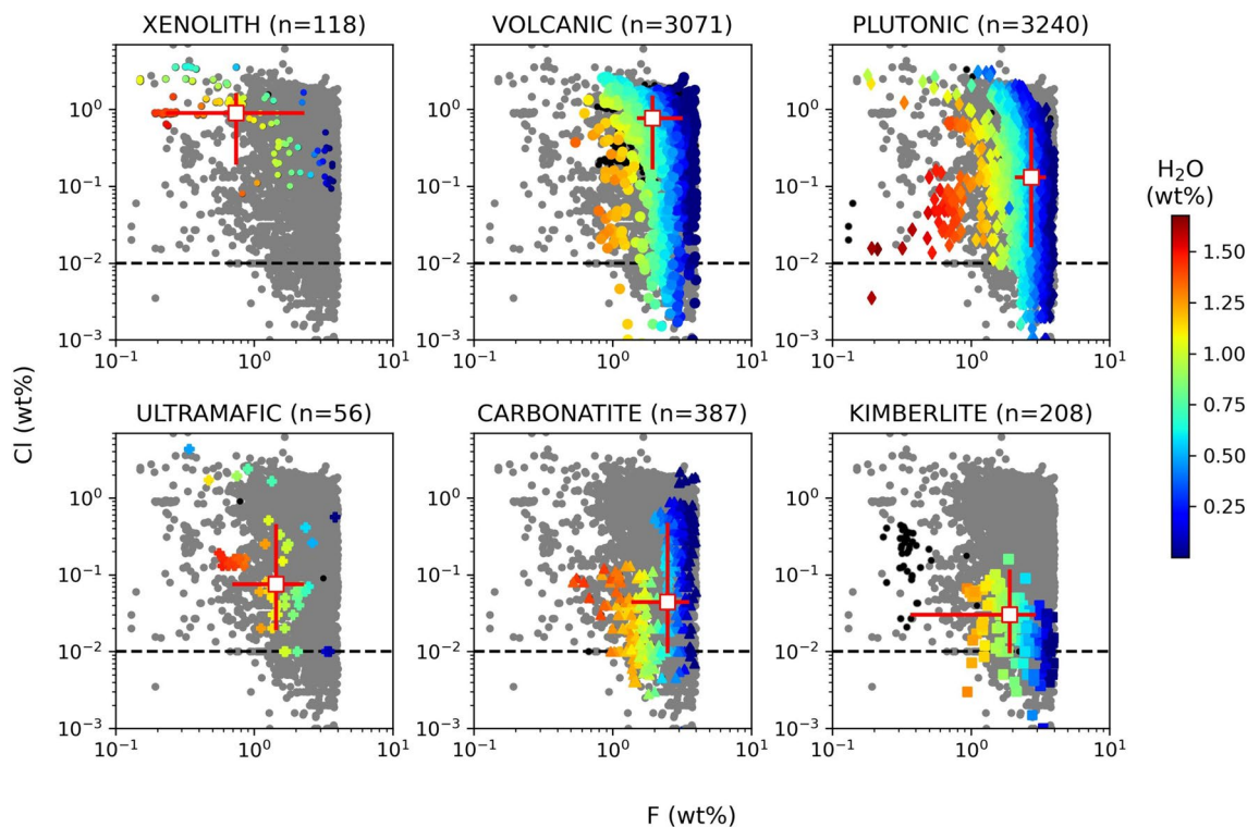
Fig. 2 F-Cl concentrations in igneous apatite from different types of rocks (with decreasing median Cl contents from the top left panel to the bottom right panel). Colors represent H 2 O concentrations calculated from stoichiometry. Data with unknown H 2 O contents are
