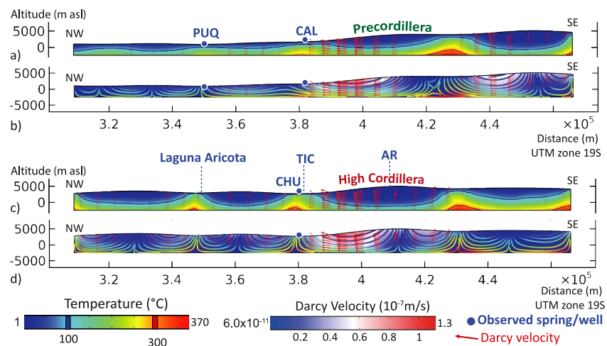
Figure 10. Heat anomalies and Darcy velocities along the Calientes and the North Incahuico fault planes for fault permeability k_f = 10^{-13} \text{ m}^2 and thickness d = 100 \text{ m} . PUQ = Puquico, CAL = Calientes, CHU = Chucutamani, TIC = Ticaco and AR = Aruma. (a) Temperatures, isotherms and orientation of the Darcy velocities along the Calientes fault, (b) Darcy velocities and flow lines colored according to the temperature along the Calientes fault, (c) Temperatures, isotherms and orientation of the Darcy velocities along the North Incahuico fault, (d) Darcy velocities and flow lines colored according to the temperature along the North Incahuico fault.
