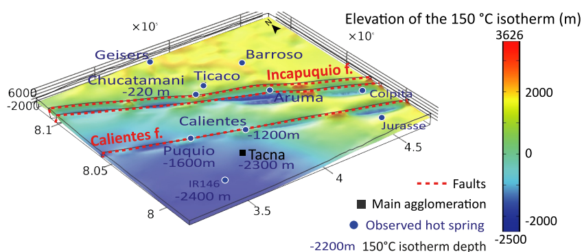
Figure 13. Elevation of the 150°C iso-surface. Blue and red zones correspond to a collapse or an upwelling of the 150°C isotherm, respectively. Blue numbers indicate the depth of the 150°C isotherm below the strategic points (see Table S6 in Supporting Information S2).
