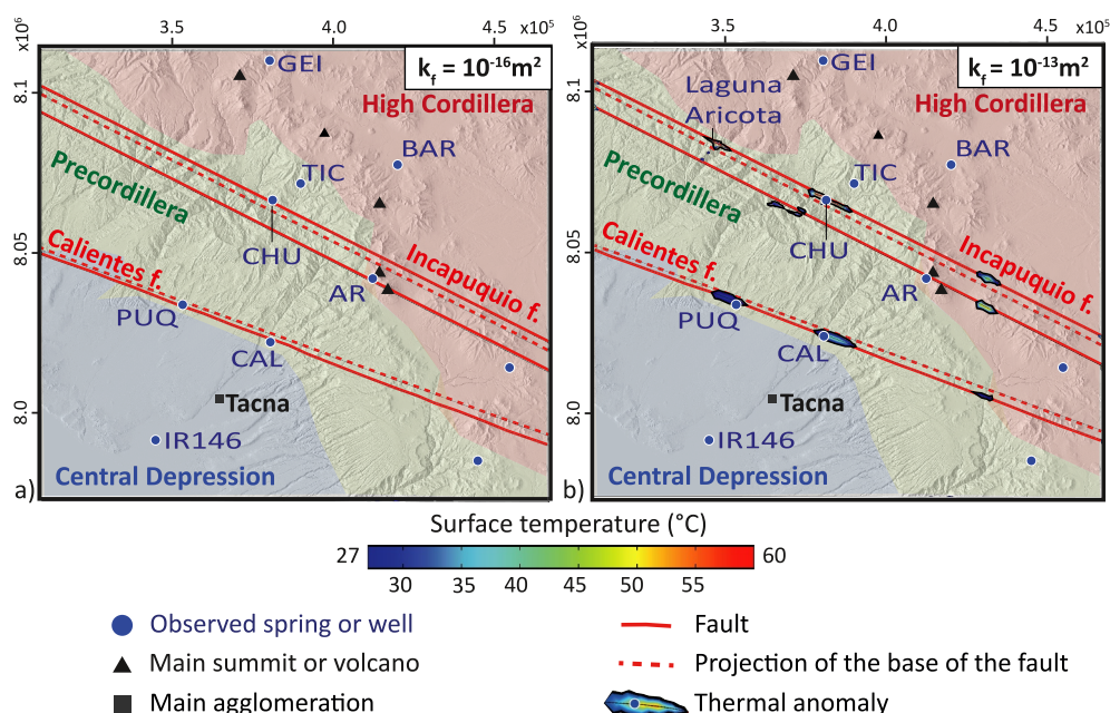
Figure 8. Thermal anomalies on the topographic surface of the numerical model, (a) for poorly permeable faults k_f = 10^{-16} \text{ m}^2 , (b) for highly permeable faults k_f = 10^{-13} \text{ m}^2 . The fault thickness d = 100 \text{ m} .
