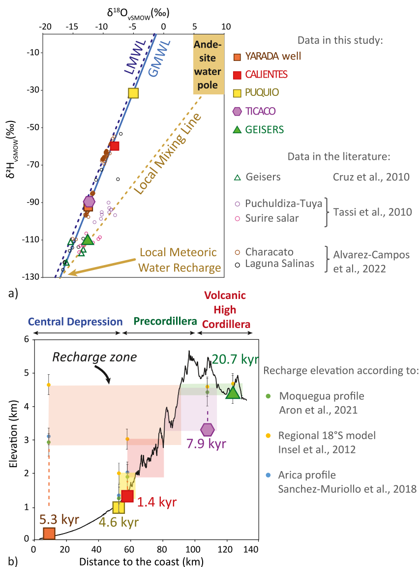
Figure 6. Isotopic composition of the thermal waters. (a) \delta^{18}\text{O} versus \delta^2\text{H} diagram with the Global Meteoric Water Line (GMWL, Craig (1961)), the Local Meteoric Water Line (LMWL, Boschetti et al. (2019)), and the Local Mixing Line linking the Local Meteoric Water Recharge (Cortecchi et al., 2005; Cruz et al., 2010) with and the Andesite (i.e., subduction arc) Water Pole (Fischer & Chiodini, 2015; Sakai & Matsubaya, 1977). Additional data on other springs nearby (Alvarez-Campos et al., 2022; Cruz et al., 2010; Tassi et al., 2010) are also represented. (b) Topographic profile between the Ocean level to the High Cordillera with the location of the springs and wells, their radiocarbon ages in kyrs and the elevation of their recharge zone calculated after Insel et al. (2012), Sánchez-Murillo et al. (2018) and P. G. Aron et al. (2021) (colored dots). The complete data set is available in Table S2 in Supporting Information S2.
