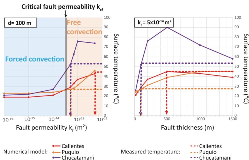
Figure 11. Temperatures measured on the model surface at the location of the Calientes, Puquiu, and Chucatamani springs as a function of, (a) the fault permeability (for a fault thickness d = 100 m, the critical fault permeability k_{cf} calculated in Section 4.2.1 separates the free and forced convection domains), (b) the fault thickness (for a fault permeability k_f = 5 \times 10^{-14} m 2 , slightly above the critical permeability). The colored arrows show parameter value allowing to reproduce the temperatures of the springs measured on the field (dot lines).
