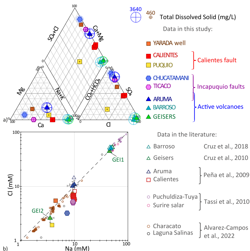
Figure 4. Composition in major ions of the thermal water. (a) Piper diagram (Piper, 1944). Colored circles represent the water Total Dissolved Solids (TDS, mg/L) and are proportional to the circles, and in the legend, (b) Na-Cl diagram (Log-log) with data from previous studies (Cruz, 2018; Cruz et al., 2010; Peña et al., 2009) and of near hydrothermal systems in the region (Alvarez-Campos et al., 2022; Tassi et al., 2010). Dotted line corresponds to Na/Cl = 1 . Complete data is available in Table S1 in Supporting Information S2 and in Taillefer et al. (2024).
