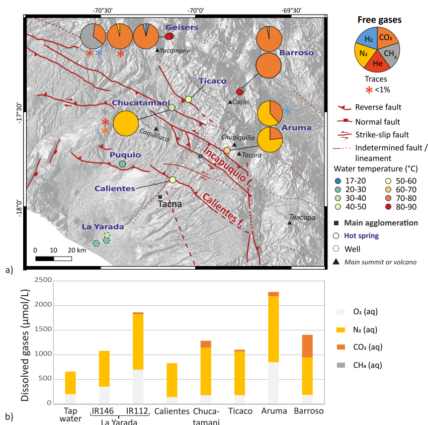
Figure 5. Gaseous composition of the thermal waters. (a) Free gases in proportion of total gases, (b) Dissolved gases concentrations in proportion of total gases. Complete data in Tables S3 and S4 in Supporting Information S2.
