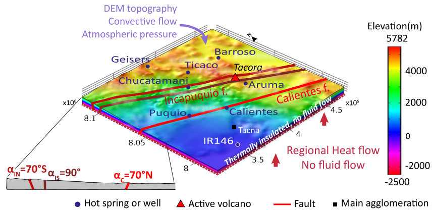
Figure 3. 3D geometry and boundaries conditions of the numerical hydrothermal model. \alpha_C , \alpha_{IN} and \alpha_{IS} correspond to dip of Calientes faults and Incapuquio North and South faults, respectively. DEM = Digital Elevation Model.
