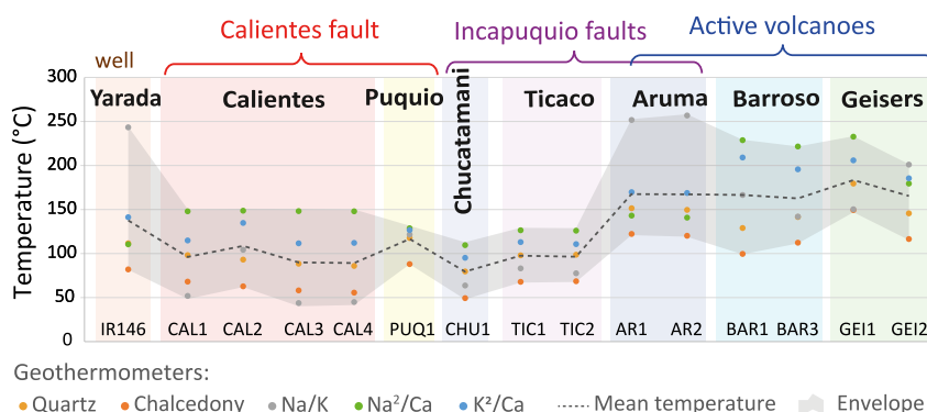
Figure 7. Reservoir temperature according to various classical geothermometers (dots, see Section 3.1.3 and Table S5 in Supporting Information S2 for details about the methodology). The mean of temperatures (dot line) and the envelope between the maximum and minimum values (gray surface) shows the general trend.
