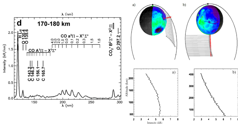
Fig. 4 From Leblanc et al. (2006) and Chaufray et al. (2008). (Left): example of spectrum observed by SPICAM in the dayside upper atmosphere of Mars at SZA between 14–37° and altitudes between 170–180 km. At these altitudes, the Lyman- \alpha hydrogen emission line (121.6 nm) becomes dominant compared to the other dayglow emissions. Right top: Example of two geometries of observations of the Martian hydrogen corona observed at high altitudes at SZA = 30° (center) and SZA = 90° above the South Pole (right). Right bottom: Associated vertical profile of the H Lyman- \alpha intensity for the two observations. Reproduced with permission; copyright by (top) Elsevier, (middle) AGU, (bottom) ESO
