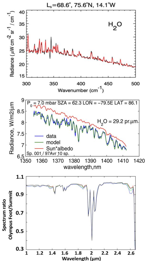
Fig. 3 Examples of spectra collected by (top) PFS (black: data, red: model) from Fouchet et al. (2007), (middle) SPICAM IR from Fedorova et al. (2006), and (bottom) OMEGA from Encrenaz et al. (2005). OMEGA spectra are given as ratios of raw spectra, with the denominator being the spectrum taken at the summit of Olympus Mons. Only the black curve is an actual observation; the other colors correspond to synthetic spectra with varying amounts of water vapor, the best fit being obtained with 150 ppmv. Reproduced with permission; copyright by (top) Elsevier, (middle) AGU, (bottom) ESO
