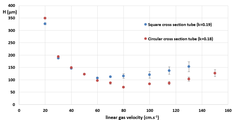
Fig. 7. Comparison of Golay plots of circular and square cross-section tubes coated with PDMS film obtained by the injection of iso -octane at 100 °C in triplicate (RSD on H values for each velocity were less than 5%).
