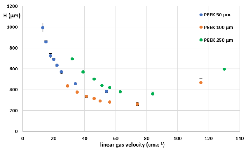
Fig. 6. Evolution of H versus the mean linear carrier gas velocity for all the junction capillaries tested by the injection of iso -octane at 100 °C in triplicate with the corresponding RSD.
