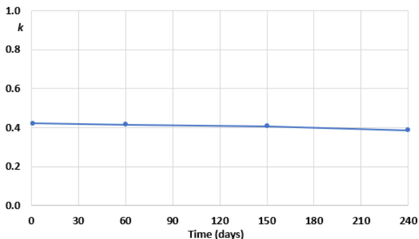
Fig. 13. Evolution of retention factor of iso -octane (average of 5 injections without measurable deviation) measured at 80 °C on microchip 6 as a function of time.
