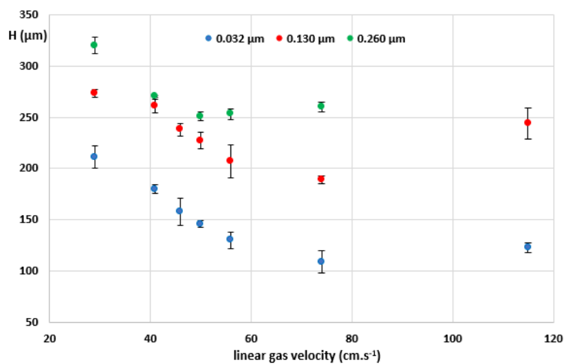
Fig. 11. Golay's plots of the three microchips detailed in Table 5 obtained by the injection of iso -octane at 100 °C in triplicate (RSD on H values for each velocity were less than 10%) d. Each curve corresponds to a PDMS film thickness.
