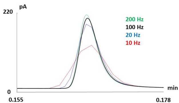
Fig. 5. Chromatographic profiles obtained by the injection of iso -octane according to conditions specified in the method and using the following data frequency acquisition (red) 10 Hz, (blue) 20 Hz, (black) 100 Hz and (green) 200 Hz.
