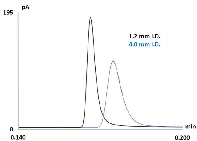
Fig. 4. Chromatograms obtained by the injection of iso -octane at 100 °C according to the conditions specified in the method with the liner of 1.2 mm I.D. (in black) and the liner of 4.0 mm I.D. (in blue).
