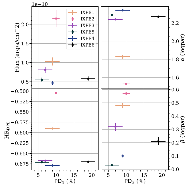
Figure 5. Various X-ray spectral properties as a function of the X-ray PD, including the IXPE 2–8 keV flux (top left), photon index \alpha (top right), IXPE 2–4 and 4–8 keV hardness ratio ( \text{HR}_{\text{IXPE}} , bottom left; see Section 4.1 for definitions), and spectral curvature (bottom right).
