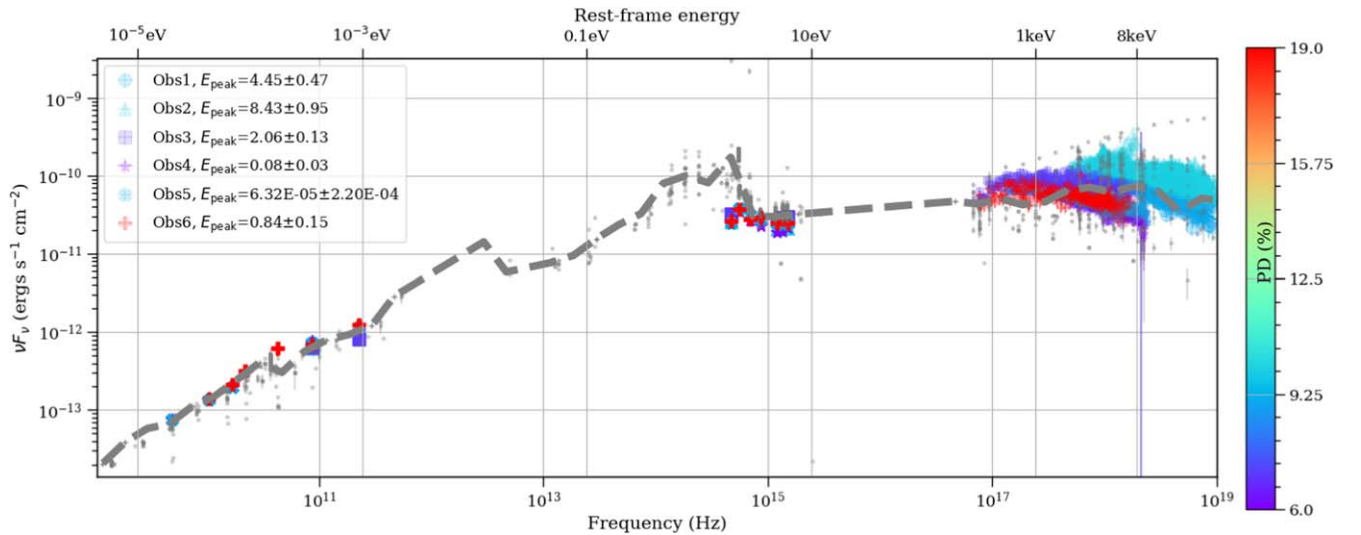
Figure 8. Broadband SED of Mrk 501, with best-fit log-parabolic model from X-ray spectropolarimetric fitting, superposed on archival data (gray points) from the SSDC SED Builder (Tramacere et al. 2009; https://tools.ssdc.asi.it/SED/ ). For comparison, we also display the archival data binned by 0.2 dex in log frequency as a dashed gray line. The vertical color bar represents the PD of each observation.
