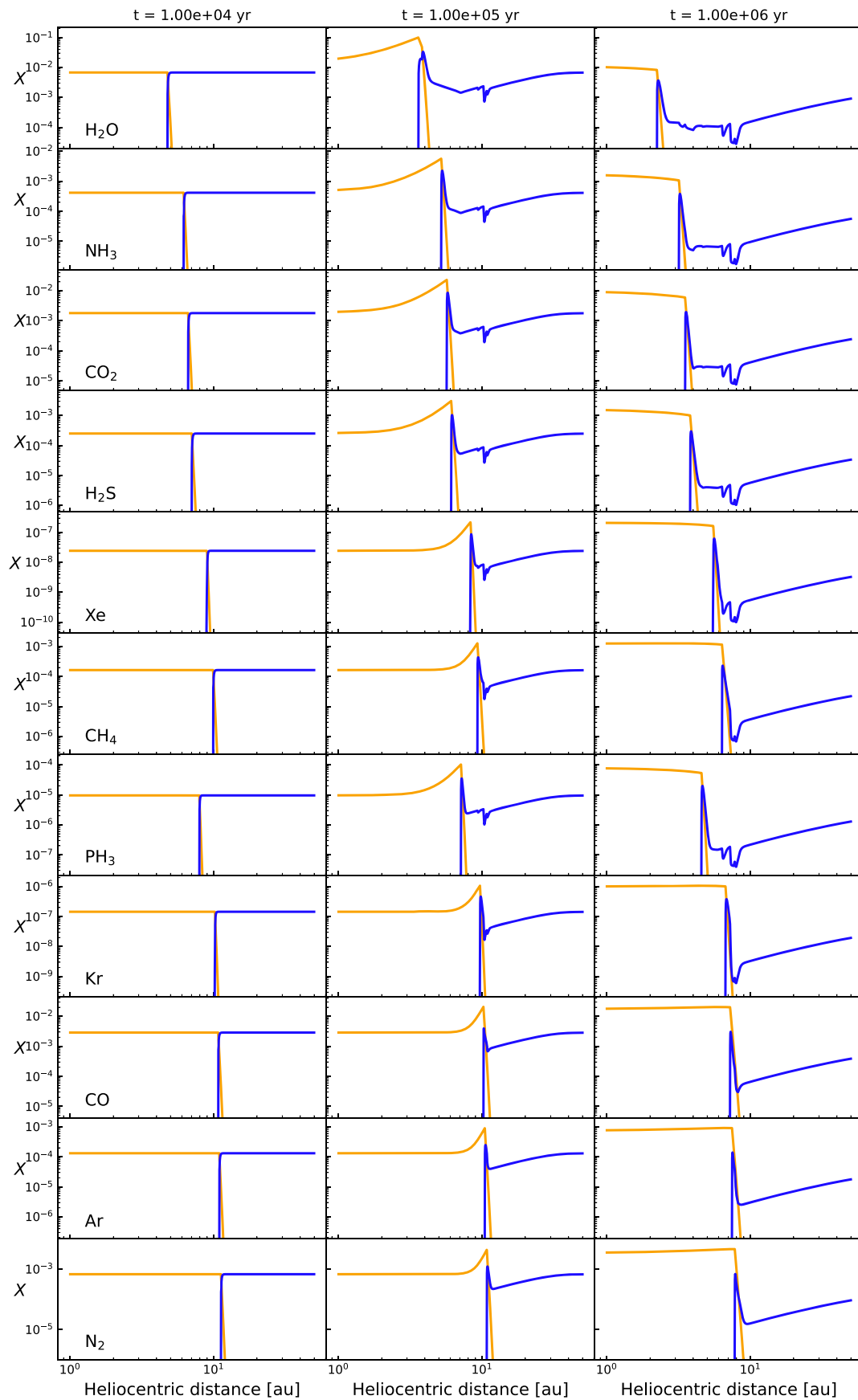
Figure 4. Molar abundance profiles of various volatile species in gaseous (orange lines) and pure condensate (blue lines) forms, calculated at different epochs (10 4 , 10 5 , and 10 6 yr) of the PSN evolution (Case 1). The species shown are H 2 O, NH 3 , CO 2 , H 2 S, Xe, CH 4 , PH 3 , Kr, CO, Ar, and N 2 .
