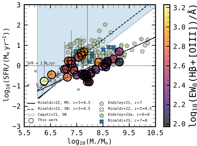
Figure 7. Location of our galaxies in the SFR– M^* plane, color coded according to their EW_0(H\beta + [O\text{ III}]) values. As in previous figures, we complement our galaxy sample with other samples from the literature at z = 5\text{--}8 (Endsley et al. 2021; Rinaldi et al. 2022; Endsley et al. 2023a; Prieto-Lyon et al. 2023; Rinaldi et al. 2023). The light-blue shaded region indicates the starburst zone, as defined in Caputi et al. (2017, 2021).
