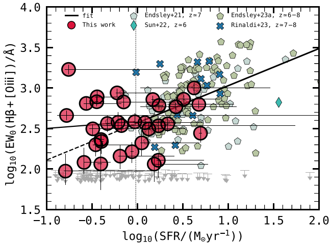
Figure 6. EW_0(H\beta + [O\text{ III}]) vs. galaxy SFR. Symbols are the same as in previous figures. The solid lines show the result of a two-component linear regression, which indicates a break in the EW_0 -SFR relation at \log_{10}(SFR/M_{\odot}\text{yr}^{-1}) = -0.02^{+0.08}_{-0.05} . The dashed line indicates the extrapolation of the higher-SFR component, which helps to show how the relation flattens out at low-SFR values. The correlation break is produced by the high dispersion observed in the low-SFR regime, with some very high EW_0(H\beta + [O\text{ III}]) values. This is likely the consequence of the dominant effect of [O\text{ III}] , and thus very low metallicities, in some galaxies with lower SFRs.
