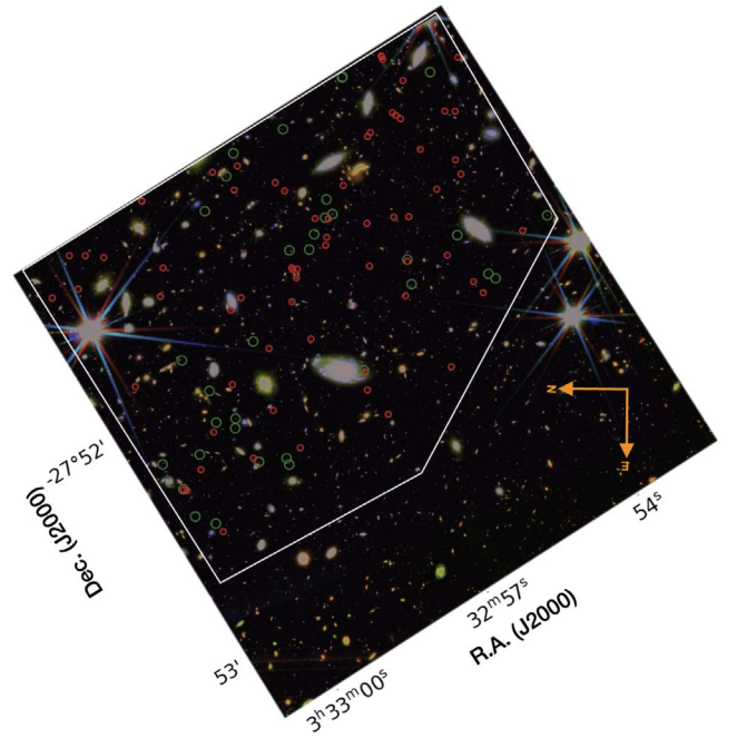
Figure 1. Red, green, and blue composite image of the P2 field with NIRCam coverage. The region delimited with a white line has the deepest coverage in the NIRCam bands and is the field considered in this work. Green circles indicate the location of our ( H\beta + [O\text{ III}] ) emitters at z = 5.5\text{--}7.0 , while the red circles correspond to all other sources in the same redshift range.
