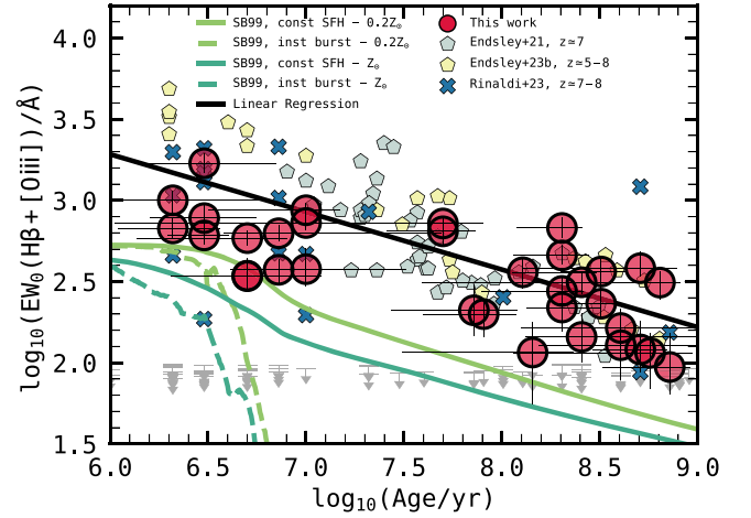
Figure 5. EW_0(H\beta + [O\text{ III}]) vs. galaxy age. We also see an anticorrelation between these two parameters, which is related to the anticorrelation observed with respect to stellar mass (see Figure 4). The solid black line corresponds to the best-fit linear regression performed on our data points along with the data from the literature. The model tracks from SB99 shown with green lines correspond only to the H\beta EW_0 and, thus, lie all below the observed data points.
