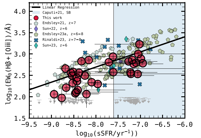
Figure 8. EW_0(H\beta + [O\text{ III}]) vs. galaxy sSFR. Symbols are the same as in previous figures. The light-blue shaded region indicates the starburst zone, as defined in Caputi et al. (2017, 2021).
