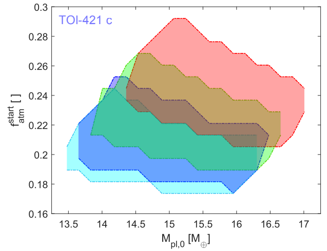
Fig. 11. Initial atmospheric mass fraction against the initial mass of the planet allowing us to reproduce the present-day parameters of TOI-421 b (top) and TOI-421 c (bottom) obtained employing the atmospheric mass fraction estimated in Sect. 6, instead of the observed radius. Notations are the same as in Fig. 10.
