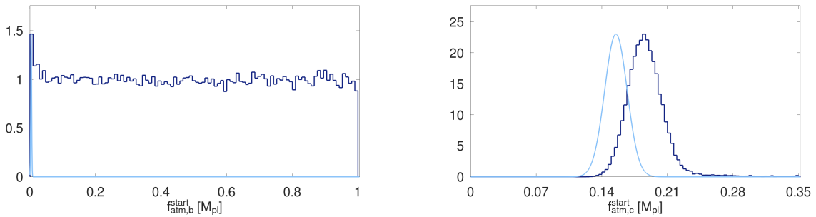
Fig. 9. Same as Fig. 8, but when fitting for the present-day atmospheric mass fraction (i.e. using the interior structure model described in Sect. 6 to convert the observed radius to the present-day atmospheric mass fraction).
