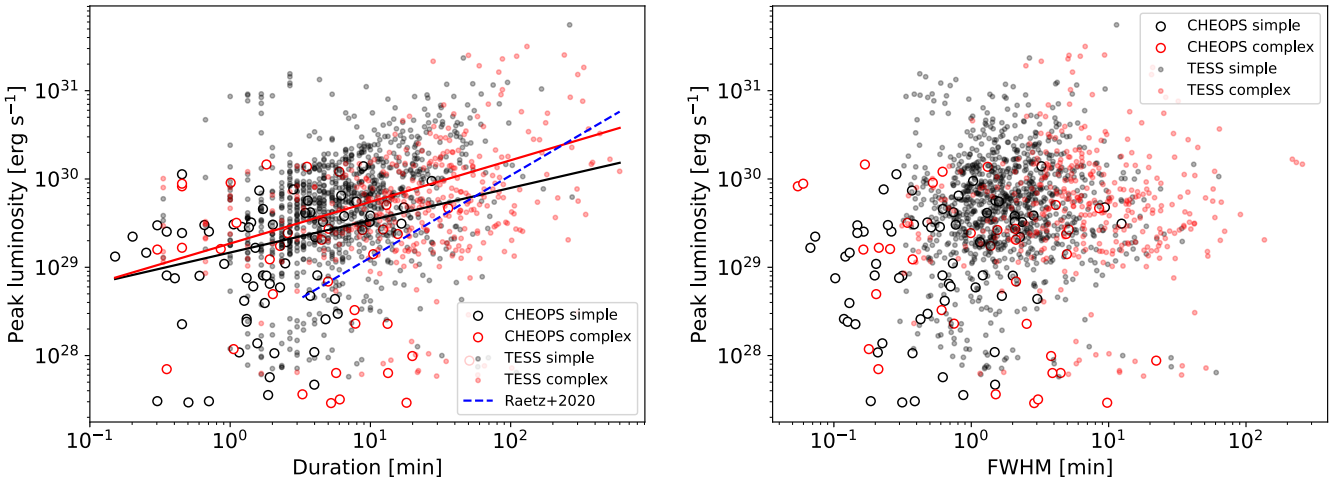
Fig. 11. Flare parameter trends. Left: relationship between flare peak luminosity and duration. Simple and multi-peak flares are separated, as well as the instrument they were detected with. The trend found by Rætz et al. (2020) is shown for the sake of comparison. Right: relationship between flare luminosity and FWHM.
