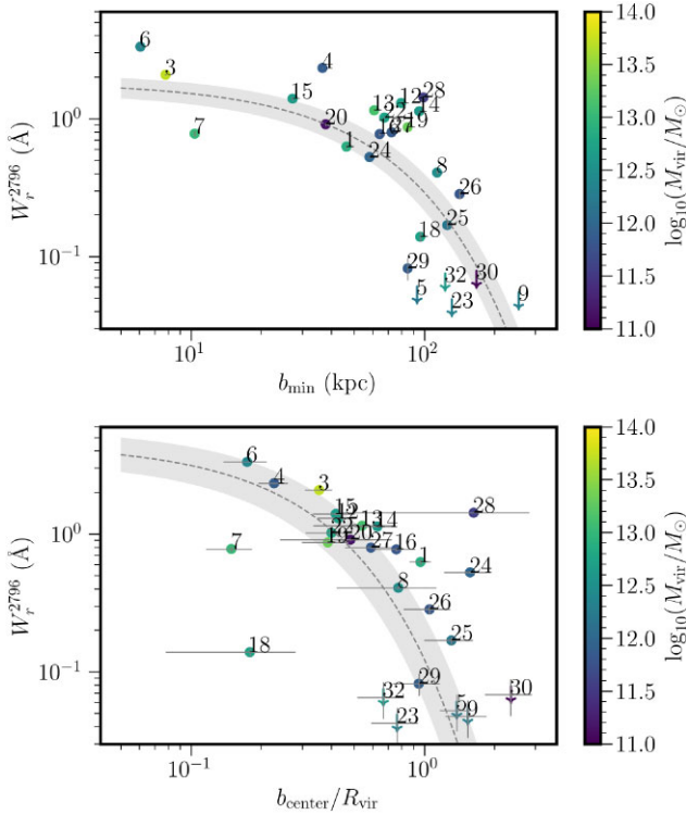
Figure 5. Top: Mg II absorption rest equivalent width versus impact parameter b to the closest galaxy and bottom: to the group centre normalized by the virial radius. The halo mass of the groups is colour coded. The groups for which no Mg II counterpart absorption system have been detected are represented by downward arrows and plotted at the detection limit. The represented error bars are 1\sigma . The grey dashed line is the best fit of the form \log_{10}(W_r^{2796}) = A \times b + B and the shaded area is the corresponding 1\sigma uncertainty.
