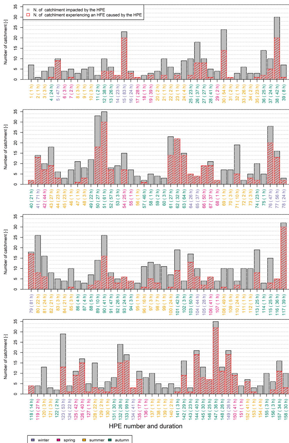
Fig. 5. number of catchment impacted by each HPE (in gray) and number of catchment that experienced an HFE caused by the HPE (portion hatched in red). The event number and duration are given on the x axis. The color of the event number corresponds to the season.
