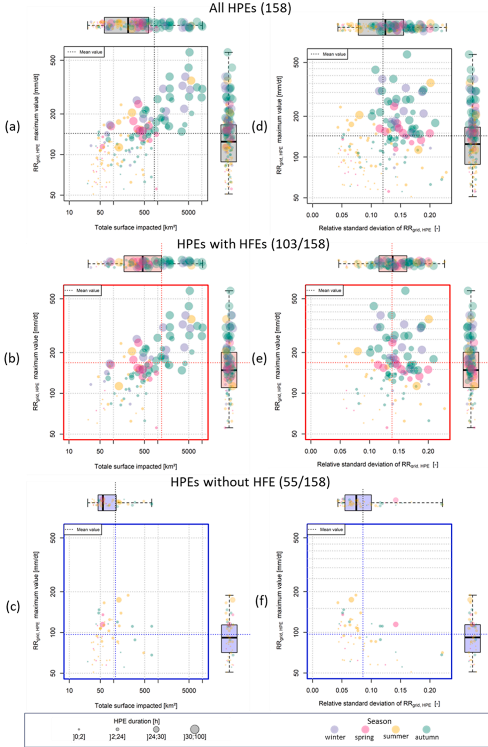
Fig. 12. (a,b,c) the maximum point precipitation accumulation as a function of the surface impacted by heavy precipitation during all the HPEs (d, e, f) the maximum point precipitation accumulation as a function of the standard deviation of the maps of precipitation accumulation. Values for all the HPEs (a, d), for HPEs with a HFE on at least one gauged catchment area (b, e) and for HPEs without HFE on gauged catchments (c, f). The size of the point varies according to the length of the episode: the longer the episode, the larger the dot. The color of the point corresponds to the season (blue dots for winter events, pink dots for spring events, yellow dots for summer events and green dots for autumn events).
