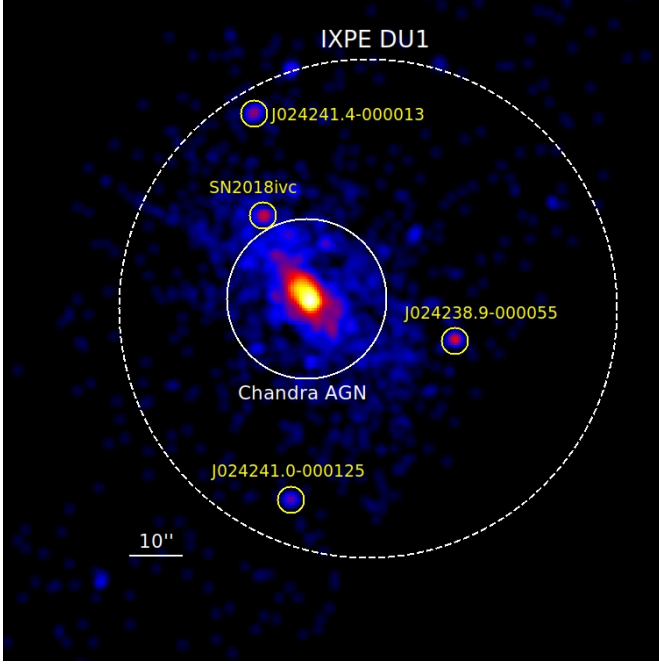
Fig. 1. 2.7 \times 2.7 central region of NGC 1068, shown in the 0.3–7.0 keV band ( Chandra ObsID 29071). The dashed white circle corresponds to the IXPE DU1 source extraction region. A Gaussian smoothing kernel of 3 \times 3 pixels has been applied for the sake of visual clarity.
