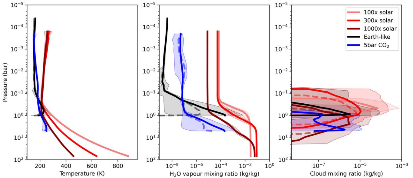
Figure E1. Results of GCM simulations of LHS 1140 b assuming mini-Neptune thick H 2 atmosphere (100×, 300×, and 1000× solar metallicity composition), an Earth-like atmosphere (1 bar N 2 , 400 ppm CO 2 ), and a thick CO 2 -dominated atmosphere (5 bar of CO 2 ). Panels show vertical profiles of the atmospheric temperatures (left), water vapor mixing ratio (middle), and water cloud mixing ratios (right). The thick solid lines indicate the global mean vertical profiles, and the dotted lines indicate the terminator vertical profiles (impacting transit spectra).
