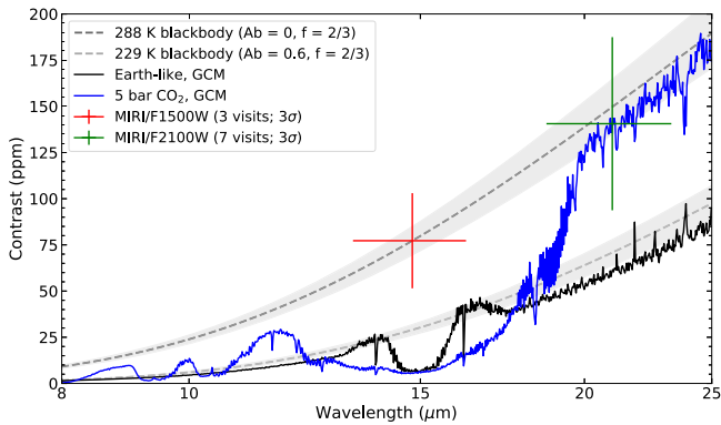
Figure 5. Predicted emission spectrum of LHS 1140 b for various scenarios, including the Earth-like (1 bar N_2 , 400 ppm CO_2 ) and pure CO_2 (5 bars) atmosphere cases from the GCMs of Cadieux et al. (2024). Extreme Bond albedo cases (0 or Europa-like) with no atmospheric heat redistribution ( f = 2/3 ) are shown with dashed lines. The gray envelope represents the 10% uncertainty of LHS 1140’s stellar flux inferred from a BT-COND model. The red plus sign, centered on the deepest airless case ( A_B = 0 , f = 2/3 ), gives the predicted uncertainty at 15 \mu m for three visits needed to reach a 3\sigma detection assuming photon-limited performance. Similarly, the green plus sign gives the number of visits needed (7) for detecting the deepest eclipse at 21 \mu m . Each visit is assumed to last \sim 7.5 hr (1 hr + 3 times the transit duration), a similar experimental design to that adopted by Greene et al. (2023) and Zieba et al. (2023) for the MIRI observations of TRAPPIST-1 b and c, respectively.
