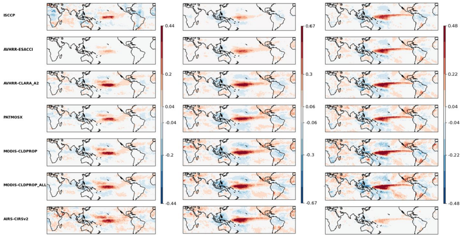
Fig. 13 Geographical maps of linear regression slopes between monthly mean anomalies in amount of thin cirrus (left), cirrus (middle) and high opaque clouds (right), relative to all clouds, and global mean surface temperature anomalies. Units are in fractional change per °C warming. Cloud data are from ISCCP, AVHRR-Cloud_cci, AVHRR-CLARA, PATMOS-x, MODIS-CLDPROP_ALL, MODIS-CLDPROP and AIRS-CIRS (from top to bottom), and surface temperature from the GISS Surface Temperature Analysis, during the period 2003–2015, 40N–40S
