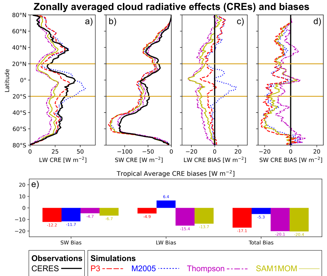
Figure 1. (a–b) Zonal average top of atmosphere cloud radiative effects (CREs) and (c–d) their biases versus CERES. Horizontal parallel lines delineate the tropical analysis region (20°S–20°N). (e) Tropical average cloud radiative effect biases for (left to right) shortwave, longwave, and total (shortwave + longwave).
