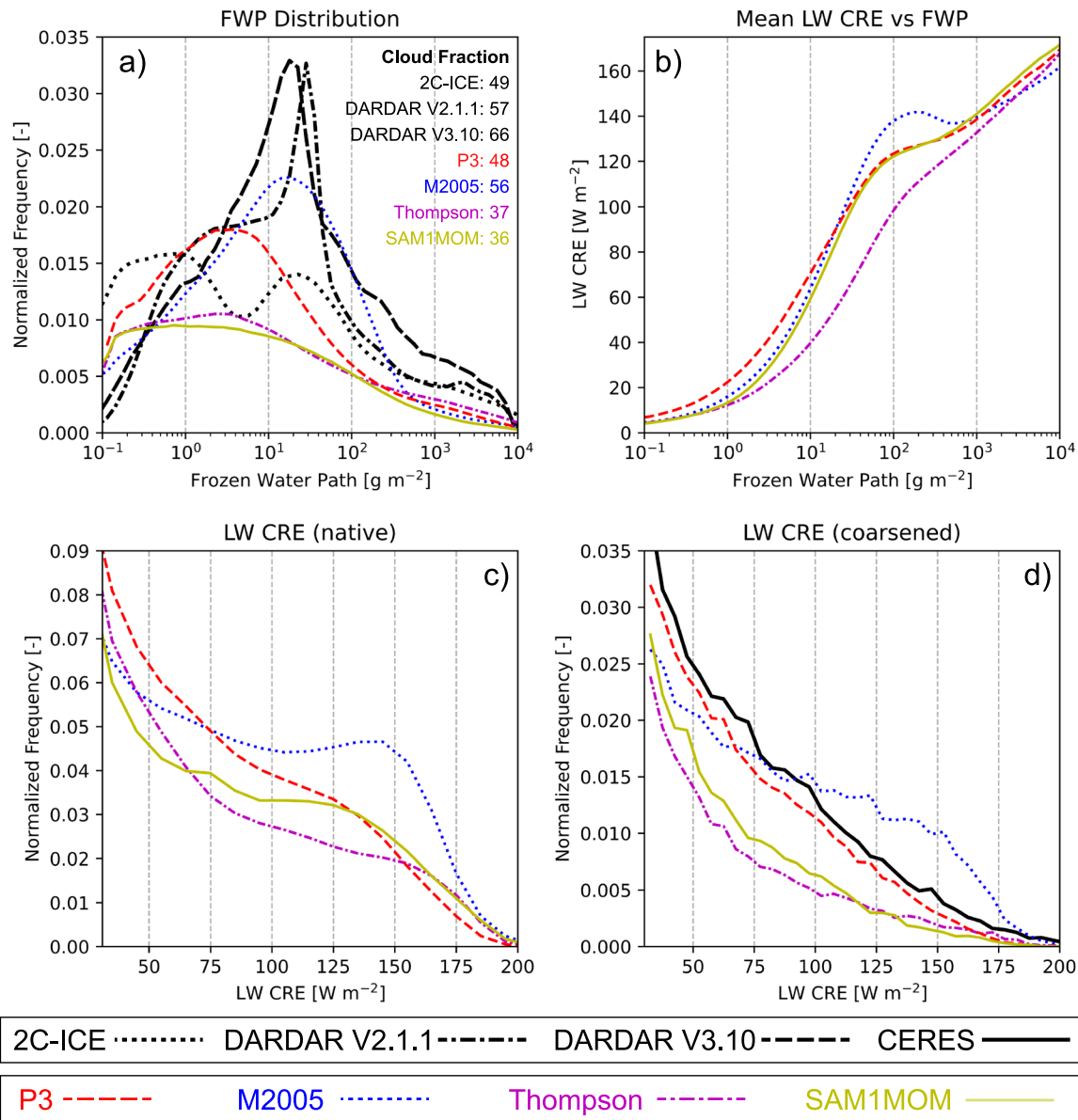
Figure 3. Tropical nighttime: (a) PDF of frozen water path (FWP) (b) Mean longwave cloud radiative effect (CRE) binned by FWP (c) PDF of longwave CRE, and (d) PDF of coarsened longwave CRE ( 1^\circ \times 1^\circ ). In panel (a), the area under the curves represents the fraction of high cloud columns, which is also printed on the plot. In panels (c and d), it represents the fraction of model columns, and 1^\circ \times 1^\circ columns, respectively, with longwave CRE > 25 \text{ W m}^{-2} .
