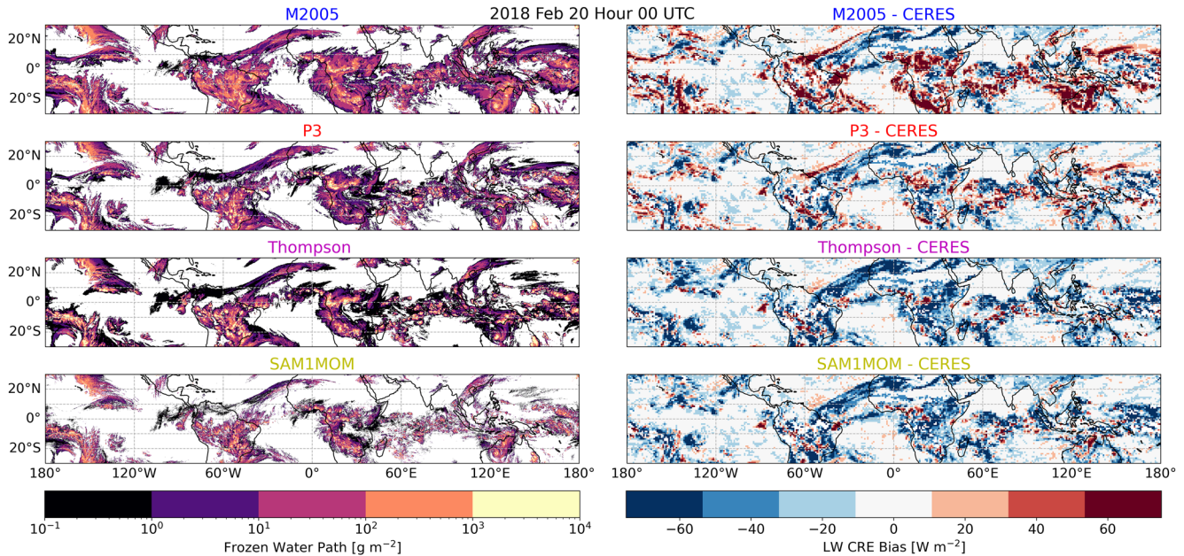
Figure 2. (left) Snapshots of simulated frozen water path for columns with CTH \geq 10 km on the simulations' native grid. (right) Coincident snapshots of longwave cloud radiative effect bias compared to CERES on a coarsened 1^\circ \times 1^\circ grid.
