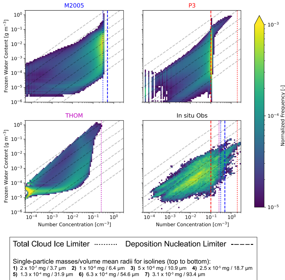
Figure 5. 2D histograms of frozen water content (y-axis, log-scale) and N_{ice} (x-axis, log-scale). Vertical dotted and dashed lines indicate limiters on total cloud ice number concentration and cloud ice particles formed through deposition nucleation, respectively. Diagonal dashed lines show isolines of volume mean radii which are listed below along with the corresponding particle mass, assuming uniformly sized spherical particles with solid ice density.
