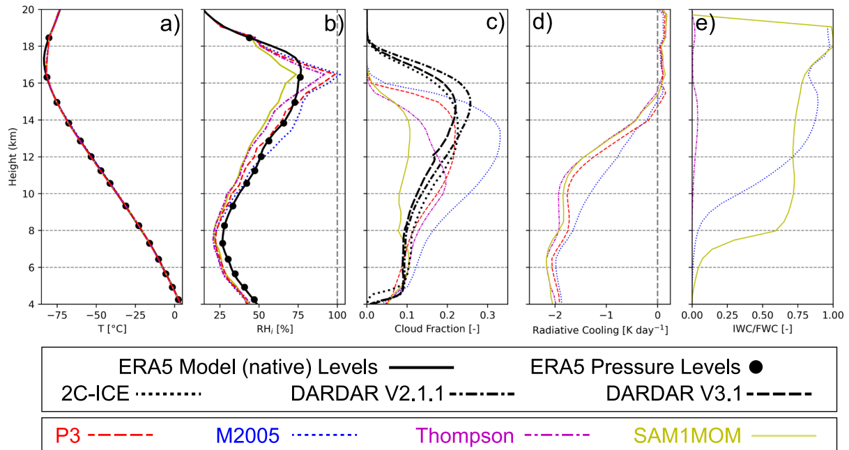
Figure 4. Vertical profiles of tropical nighttime (a) median temperature, (b) median RH_i , (c) cloud fraction (frozen water content (FWC) \geq 10^{-4} \text{ g m}^{-3} only), (d) mean longwave radiative cooling, and (e) IWC/FWC. We run P3 with one ice class so IWC/FWC cannot be computed.
