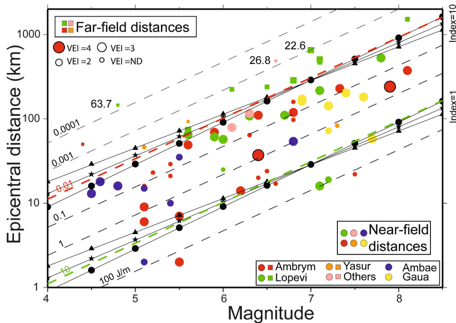
Fig. 5. Distribution of the volcanic activity changes plotted in a \log_{10} -linear axis of the epicentral distance versus magnitude M corresponding to the Vanuatu volcanoes of Table 1. The different colors correspond to the different volcanoes. “Others” correspond to the Karua and Epi volcanoes. Colored dots correspond to near-field earthquake-volcano distances (index \leq 10 ) and colored squares to far-field distances (index > 10 ). We added the theoretical maximum distance curves (black lines) for each magnitude corresponding to normal (triangle), reverse (circle) and strike-slip (asterisk) focal mechanism, for an index of 10 and an index of 1. The size of the symbols defines the VEI. The smaller size corresponds to volcanic changes that are not explosions and for which the VEI are not defined (VEI=ND). The grey dashed lines correspond to the contours of constant seismic energy density e (in \text{J}/\text{m}^3 ) varying from 0.0001 to 100 \text{J}/\text{m}^3 . The red dash line corresponds to e = 0.01 \text{ J}/\text{m}^3 crossing the three black lines of Index = 10 and the green dash line corresponds to e = 10 \text{ J}/\text{m}^3 crossing the three black lines of Index = 1. (For interpretation of the references to color in this figure legend, the reader is referred to the web version of this article.)
