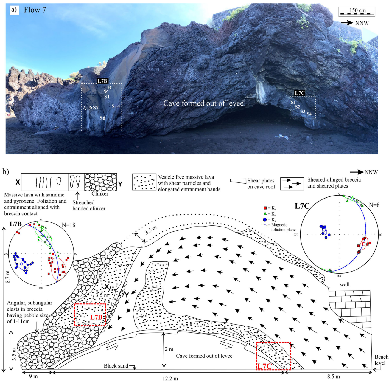
Fig. 3 a Field photo of channel at Flow 7 above the Grotta di Eolo, showing two sampling location (site L7B and L7C) marked with dotted rectangular lined. b Sketch of master channel with AMS results. The top flow is partially eroded above the cave, as evidenced by the
