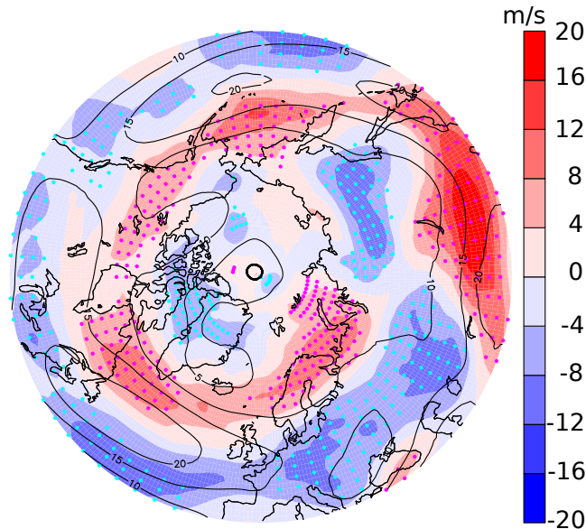
FIG. 3. Zonal wind anomaly at 300 hPa in August 2022 (shadings; units: \text{m s}^{-1} ) with respect to the 1979 to 2022 August climatology (contours; interval: 10 \text{ m s}^{-1} ). Purple and light blue dots respectively correspond to positive and negative anomalies larger than the standard deviation. Data from ERA5 monthly reanalysis with 1^\circ \times 1^\circ grid spacing (Hersbach et al. 2020).
