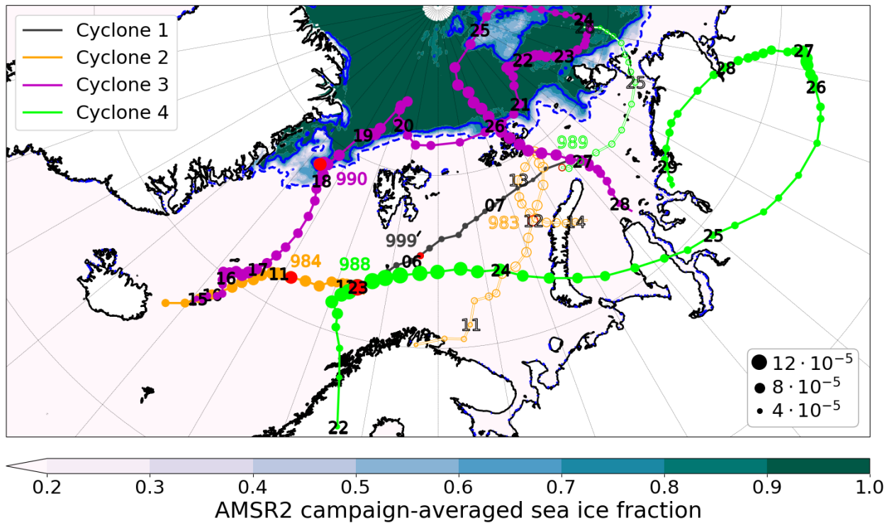
FIG. 4. Tracks of the four Arctic cyclones observed during THINICE. Cyclones locations are displayed with three-hourly frequency. Black date stamps (days in August 2022) are overlaid on the 00 UTC cyclone location. Location dot size is proportional to the 850-hPa relative vorticity ( s^{-1} ). Red dots indicate the time of maximum relative vorticity and the value of minimum MSLP (hPa) at the same time is displayed near the track. Secondary cyclones associated with Cyclones 2 and 4 are shown with the same colours as their primary counterparts, but with open circles. Tracks and cyclone intensities are based on ERA5 datasets. Advanced Microwave Scanning Radiometer 2 (AMSR2) sea ice fraction (Spreen et al. 2008) averaged between 29 July and 25 August is shaded, with solid and dashed blue contours respectively indicating values of 0.8 and 0.15, the limits of pack and marginal ice.
