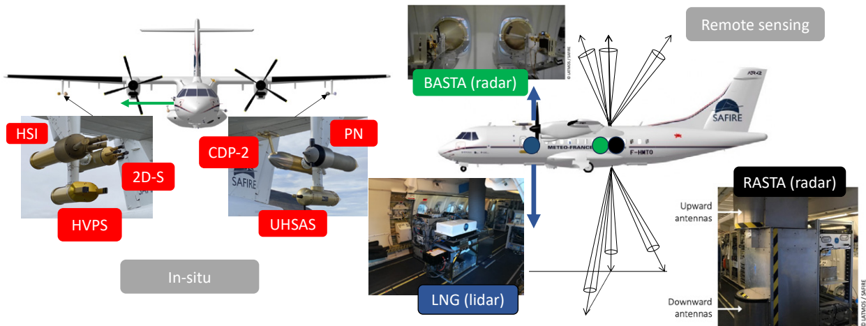
FIG. 1. Schematic of the Safire ATR42 aircraft configuration and payload: (left) in-situ microphysical probes shown in red, (right) remote-sensing instruments (positions of BASTA and RASTA radars and LNG lidar are indicated in green, black and blue respectively). Acronyms are defined in Table 1.
