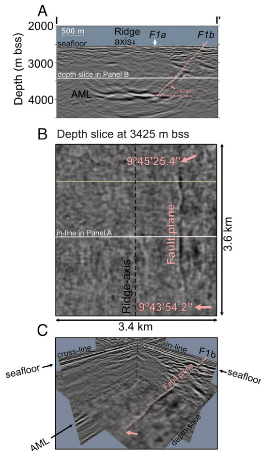
Fig. 4. Imaging fault plane in the seismic volume. (A) Seismic section extracted from the volume in cross-axis direction (i.e., inline; location marked in Fig. 2B) showing the presence of the AML and ridge ward dipping reflection signal in the upper crust, we interpret as a fault plane, F1b. In white arrow, we mark the surface location of the F1a. (B) The depth slice extracted from the volume at 3,425 m below the sea surface showing continuous linear feature, we interpret as fault plane, delimited by pink arrows. The intersections between the inline (panel A) and depth slice (panel B) are indicated in white horizontal lines in both panels. The ridge axis is marked in black dashed line. The yellow line does not have interpretation significance—it marks the merging front of two parts of the volume uploaded separately due to graphic memory limitations. (C) Intersections between inline, depth slice, and crossline (ridge parallel direction) to emphasize the linearity of the reflector (marked in pink line) and provide evidence against the possibility for the event to represent diffraction tail artifact. The same panels without interpretation are shown in SI Appendix , Fig. S3.
