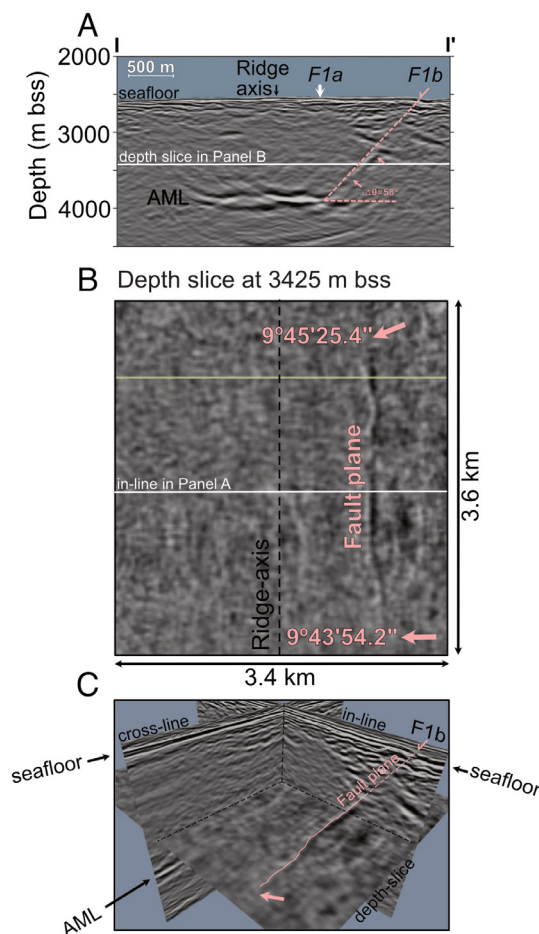
Fig. 4. Imaging fault plane in the seismic volume. (A) Seismic section extracted from the volume in cross-axis direction (i.e., inline; location marked in Fig. 2 B ) showing the presence of the AML and ridge ward dipping reflection signal in the upper crust, we interpret as a fault plane, F1b . In white arrow, we mark the surface location of the F1a . (B) The depth slice extracted from the volume at 3,425 m below the sea surface showing continuous linear feature, we interpret as fault plane, delimited by pink arrows. The intersections between the inline (panel A) and depth slice (panel B) are indicated in white horizontal lines in both panels. The ridge axis is marked in black dashed line. The yellow line does not have interpretation significance—it marks the merging front of two parts of the volume uploaded separately due to graphic memory limitations. (C) Intersections between inline, depth slice, and crossline (ridge parallel direction) to emphasize the linearity of the reflector (marked in pink line) and provide evidence against the possibility for the event to represent diffraction tail artifact. The same panels without interpretation are shown in SI Appendix , Fig. S3.
