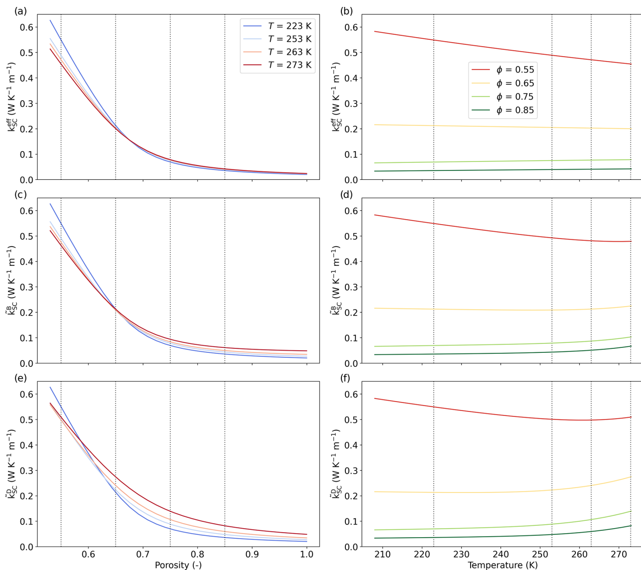
Figure 5. Evolution of the SC estimates of the thermal conductivities k_{SC}^{eff} , \tilde{k}_{SC}^B , and \tilde{k}_{SC}^D with respect to porosity at four temperatures ( a , c , e ) and with respect to temperature for four porosities ( b , d , f ). The vertical dotted gray lines indicate the four temperature and porosity values considered.
