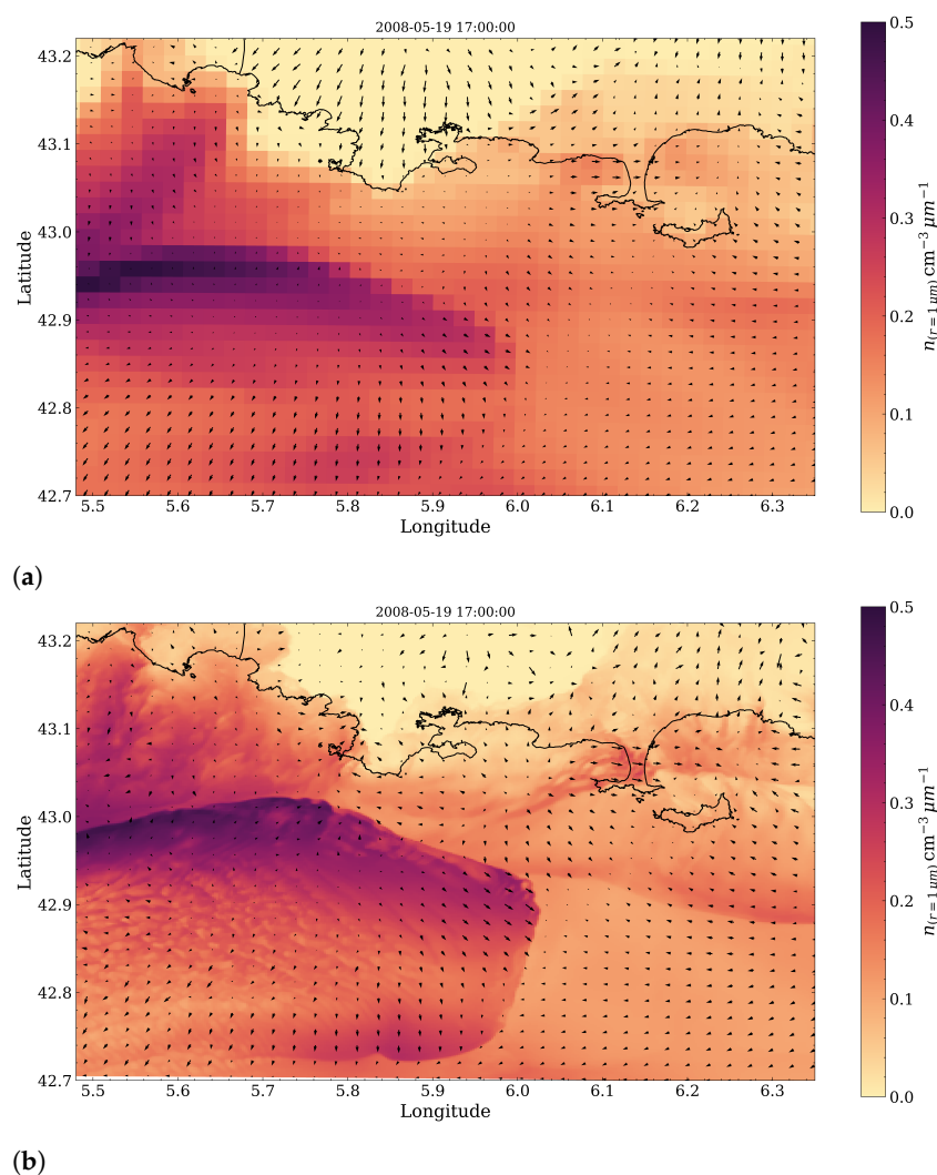
Figure 13. Map of sea-spray concentration calculated using the MesoNH (a) and the MesoNH LES (b) model for the day of 19 May at 5 p.m.
