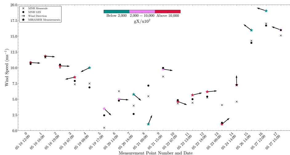
Figure 7. A comparison of the wind speed measurements taken on board the R/V Atalante (stars symbols) with the numerical simulations from both the mesoscale model (crosses) and the high-resolution model (bullets). The numbers on the x-axis correspond to the measurements points as shown in Figure 1. The colour of the stars indicates the calculated non-dimensional fetch (Equation (1)) as shown in the horizontal colour bar reported on the top of the figure. We also reported the wind direction recorded during each episode.
