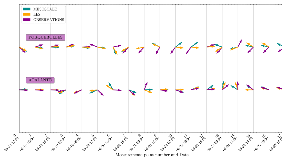
Figure 10. Comparison of wind directions from Meso-NH mesoscale and Meso-NH LES configurations with measurements at the Porquerolles site and for the MIRAMER campaign.
