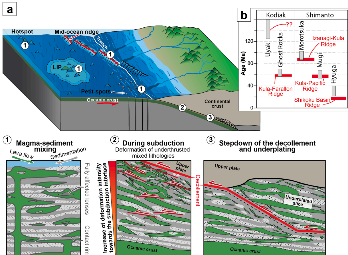
Fig. 5. (a) Model of mélange evolution from deep seafloor down to the base of the accretionary prism. (1) Basalt-sediment mixing on the ocean floor occurs in a variety of contexts: hotspots, large igneous provinces (LIP), petit-spots, and mid-ocean ridges. (2) Underthrust sequence experienced varying degrees of deformation intensity depending on its proximity to the subduction interface. (3) Steppedown of the decollement and underplating of mélange slices. (b) Deposition ages of each mélange from the Kodiak complex and the Shimanto Belt (gray boxes), with previously proposed ridge subduction events in both complexes (red boxes).
