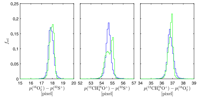
Fig. 4. Probability distributions of the differences in position of the 3 peaks in the m_c/z = 32 mass spectra (blue for channel A, green for channel B).
