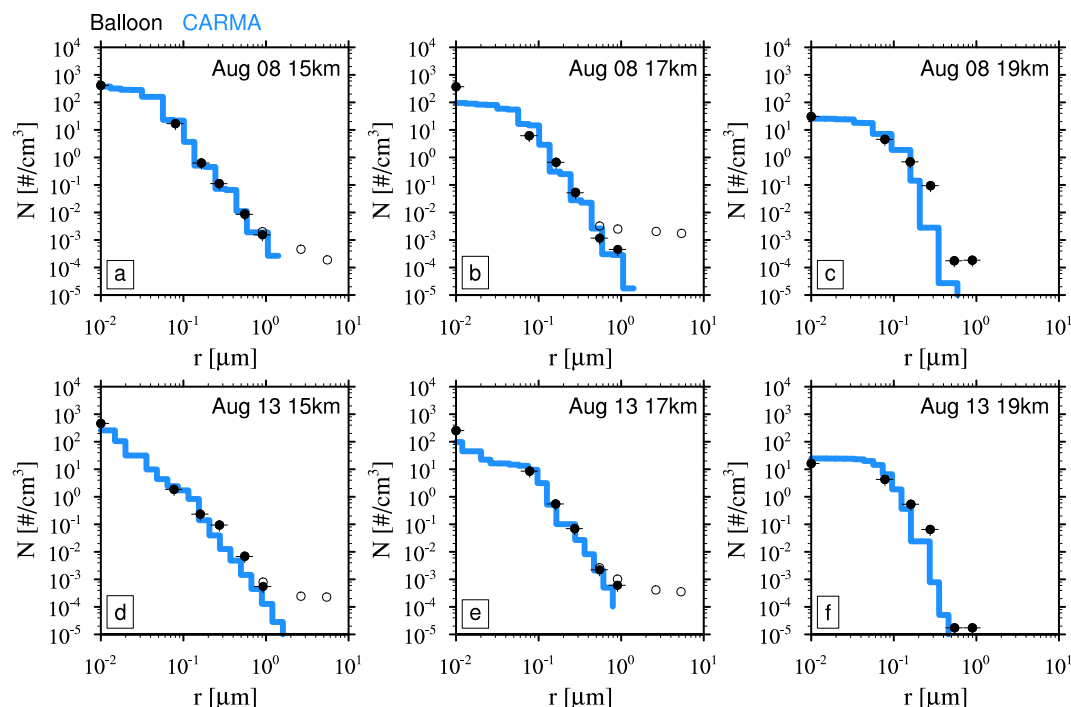
Figure 7. The number concentrations that are larger than a particular radius from the BATAL balloon observation over Hyderabad, India ( 17^\circ\text{N} , 78^\circ\text{E} ) (black dots), and from the model at the nearest location ( 18^\circ\text{N} , 77.5^\circ\text{E} ) (blue line). Black rimmed circles are the original observations including both aerosol and cloud particles. The black dots eliminate particles with diameter > 3 \mu\text{m} .
