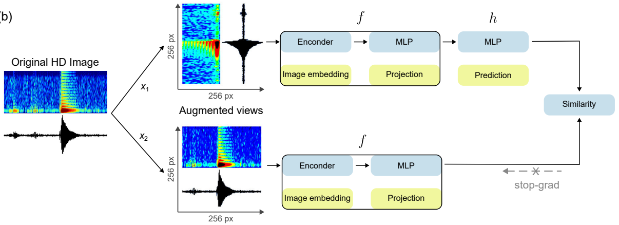
Figure 2. (a) Flowchart of the clustering workflow from the input images to the final clusters. The workflow uses three algorithms: SimSiam which is the SSL network; t-SNE (t-distributed stochastic neighbors embedding) as a dimension reduction tool and DBSCAN (density based spatial clustering of application with noise) for clustering application. (b) Architecture of the SimSiam network (after Chen & He (2021), figure 1). x_1 and x_2 represent the two augmented views of the original high dimension image. f is an encoder network, composed of an encoder and a projection multi layer perceptron. x_1 and x_2 are processed by the same encoder network f . The prediction MLP h is then applied on one side. On the other side, a stop-gradient operation is applied. Finally the model maximizes the similarity between both sides.
