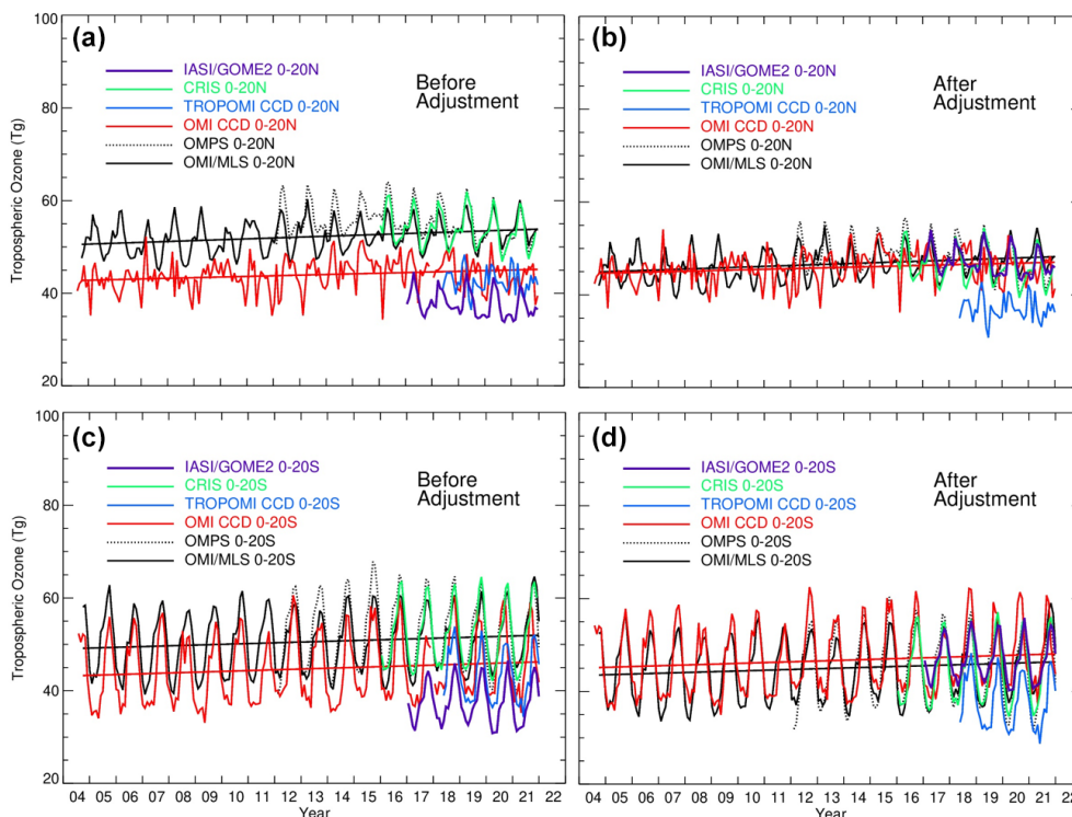
Figure 8. Time series of tropospheric ozone burden ( T_g ) from OMI/MLS, OMPS/MERR2, OMI CCD, TROPOMI, CrIS, and IASI/GOME2. The panels show the monthly means for the Northern Hemisphere ( a , b ) and the Southern Hemisphere ( c , d ) before and after bias correction. The biases we used are in Dobson units (DU) and from the differences between IASI/GOME2 and TROPOMI TCO using the reference TCO up to 270 hPa and between OMI, OMI/MLS, OMPS/MERRA-2, CrIS, and TCO using the reference TCO up to 150 hPa (Figs. 4 and 5).
