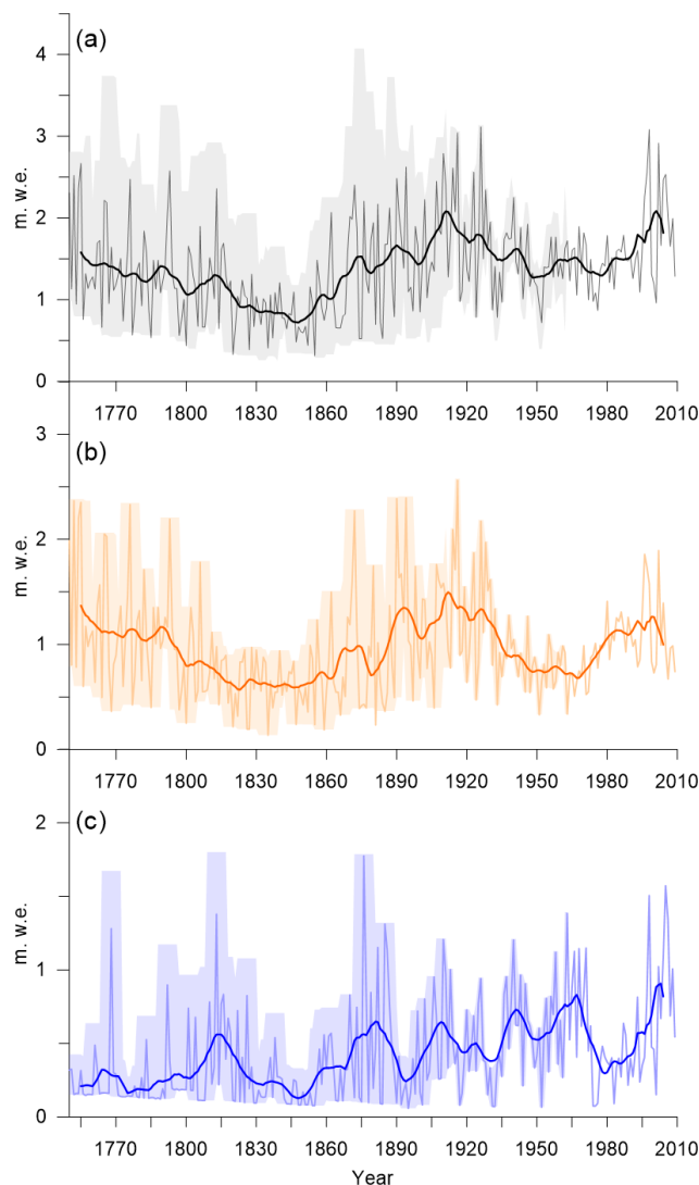
Figure 4. Reconstructed annual (a), summer (b), and winter (c) snow accumulation at the WP. The 10-year moving averages are shown as thick lines. Uncertainties are shown as shaded areas.
