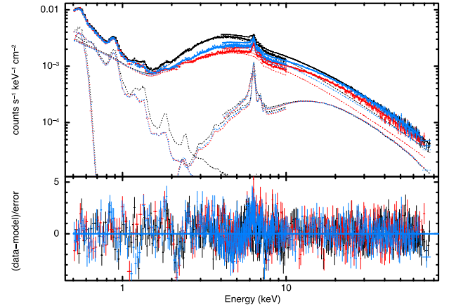
Fig. 3. XMM-Newton and NuSTAR spectra with residuals. The XMM-Newton /EPIC-pn and the grouped NuSTAR FPMA and FPMB of the first campaign are shown in black. In red, the XMM-Newton /EPIC-pn and the grouped NuSTAR FPMA and FPMB of the second campaign (first segments) are shown. In blue, the XMM-Newton /EPIC-pn and the grouped NuSTAR FPMA and FPMB of the second campaign (second segments) are presented.
