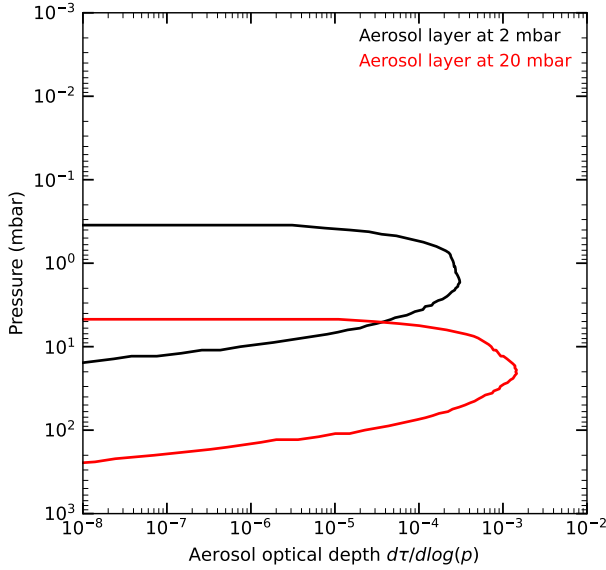
Fig. 9. Retrieved aerosol optical depth profile at 69^\circ\text{S} for the spectral interval from 700 to 701\text{ cm}^{-1} . In the black profile we assumed model A* ( 2\text{ mbar} ) and in the red one we assumed model B* ( 20\text{ mbar} ).
