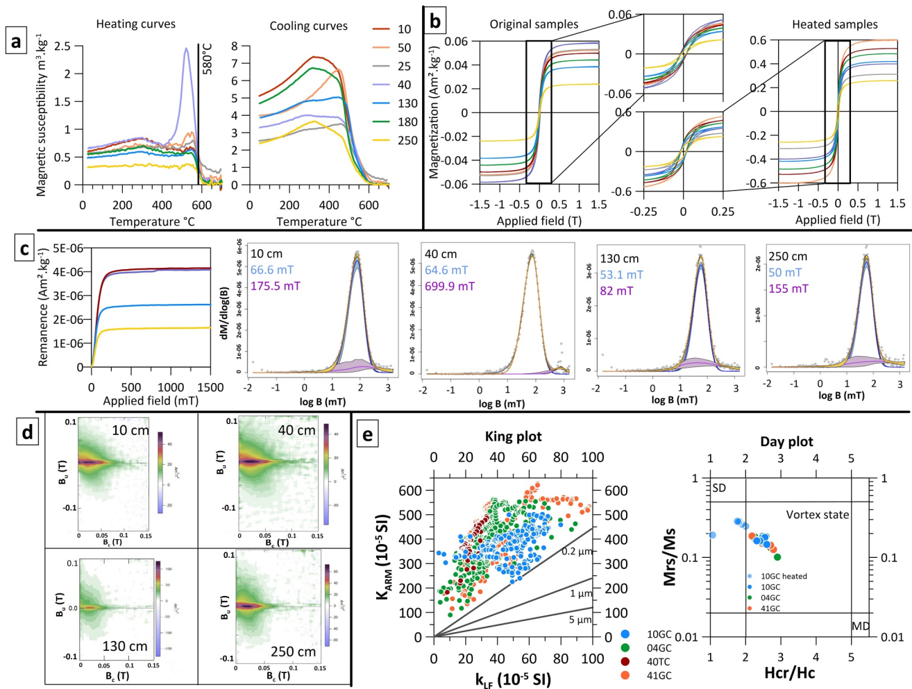
Figure 3. Rock magnetic analysis results. (a) Magnetic susceptibility heating and cooling thermomagnetic curves. (b) Hysteresis loops of samples before and after heating to 700°C. (c) Isothermal remanent magnetization (IRM) acquisition curves and IRM unmixing. (d) FORC diagrams. (e) Day & King plots.
