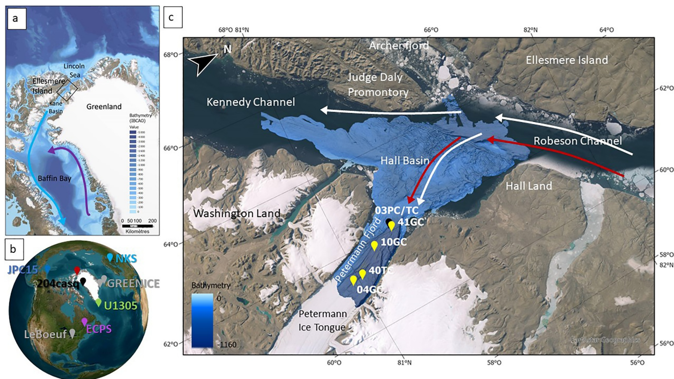
Figure 1. (a) Location of study site in Nares Strait, with bathymetric data from the International Bathymetric Chart of the Arctic Ocean (IBCAO, Jakobsson et al., 2020). Blue arrows represent the cold polar waters becoming the Baffin Current, Purple arrows represent the West Greenland Current. (b) Location of the comparison records mentioned in this study. (c) Map of the study sites in Petermann Fjord. Multibeam bathymetry of the Petermann Fjord and Hall Basin were obtained from Jakobsson et al. (2018). Black dots = cores composing the outer fjord splice; yellow dots = cores composing the stack. 10GC was collected during AMD1902 expedition (REF), 03PC/TC, 41GC, 04GC, 40TC during OD1507 (Reilly et al., 2019). Surface Polar Waters are represented by white arrows and subsurface Atlantic Waters are represented by red arrows.
