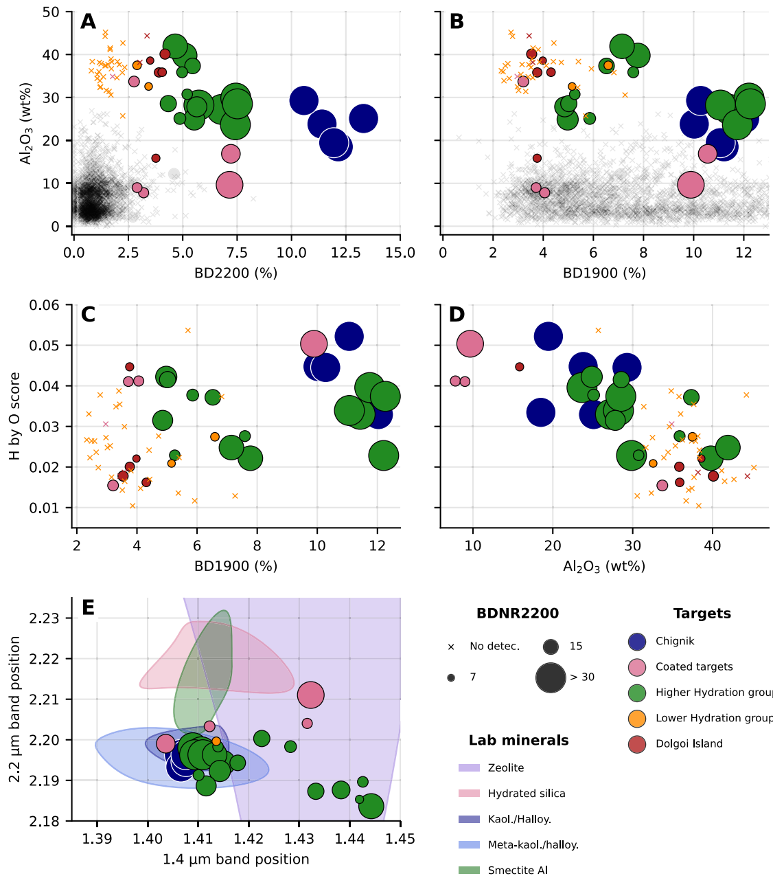
Fig. 5 | LIBS \text{Al}_2\text{O}_3 and H-content compared to the IR hydration band depths, and band positions. \text{Al}_2\text{O}_3 content compared to band depth of the 2.2 \mu\text{m} band A and the 1.9 \mu\text{m} band B . H score (normalized by the oxygen line) of the studied targets as a function of 1.9 \mu\text{m} band depth C and \text{Al}_2\text{O}_3 content D . E shows the relationship between the 1.4 (Al-OH, \text{H}_2\text{O} ) and 2.2 \mu\text{m} (Al-OH, Si-OH) bands. The corresponding relation for lab minerals is indicated as colored patches, highlighting
