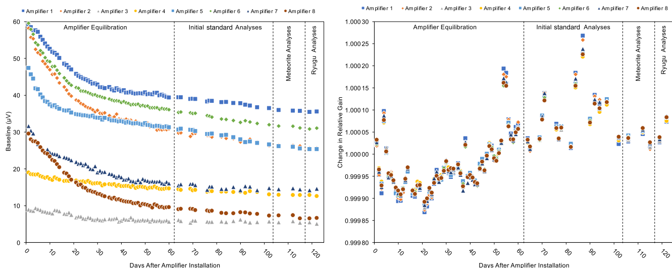
FIGURE 1. The electronic baseline (left) and the change in relative gain (right) performed with 10^{13} \Omega amplifiers using the 3.3 pA calibration board from the time of amplifier installation through the time of Ryugu sample analyses. The change in relative gain is calculated by dividing the individual amplifier relative gains returned from the gain calibration procedure by the average of all the relative gains reported for that amplifier during the time window of these measurements. Dashed lines separate the periods of amplifier equilibration, initial standard analyses, meteorite analyses, and Ryugu sample analyses. Standards were also measured throughout the meteorite and Ryugu sample analysis periods. The factory installed ninth amplifier used in this study, which was in the amplifier housing since delivery and installation in February 2019, had somewhat different baseline and gain values and is not shown in this figure. Its average baseline was -13 \mu\text{V} with a total drift of 6 \mu\text{V} over the time window shown in this figure, and its change in relative gain closely matched those of the other amplifiers. (Color figure can be viewed at wileyonlinelibrary.com )
