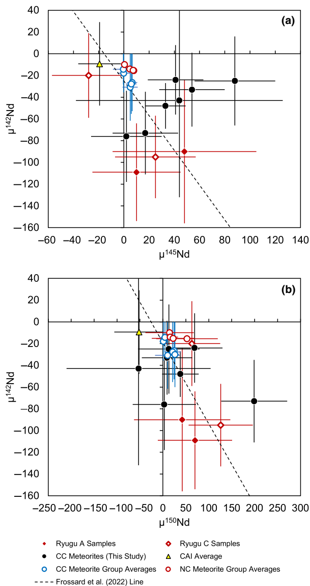
FIGURE 3. (a) \mu^{142}\text{Nd} versus \mu^{145}\text{Nd} and (b) \mu^{142}\text{Nd} versus \mu^{150}\text{Nd} for Ryugu “A” (solid red diamonds) and “C” (open red diamonds) samples and carbonaceous chondrites (black circles) from this study and CC (open blue circles) and NC (open red circles) meteorite group averages (Burkhardt et al., 2016; Frossard et al., 2022; Fukai & Yokoyama, 2017, 2019; Render & Brenneka, 2021; Saji et al., 2020) and the CAI average (yellow triangle; Brenneka et al., 2013; Bouvier & Boyet, 2016; Burkhardt et al., 2016; Shollenberger et al., 2018) from previous studies. The dashed r-, s-process mixing line represents high-precision measurements of leaches of Orgueil (Frossard et al., 2022). (Color figure can be viewed at wileyonlinelibrary.com )
