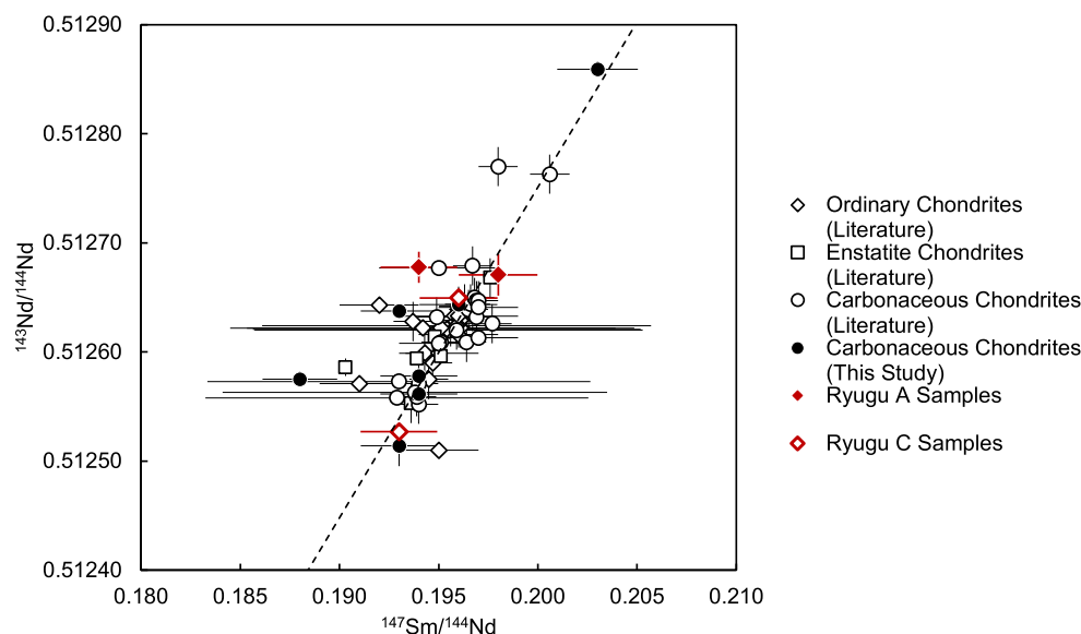
FIGURE 4. ^{147}\text{Sm} – ^{143}\text{Nd} isochron diagram including data for Ryugu “A” (solid red diamonds) and “C” (open red diamonds) samples and carbonaceous chondrites (black circles) measured in this study and ordinary chondrites (white diamonds; Bouvier et al., 2008; Boyet & Carlson, 2005; Fukai & Yokoyama, 2017), enstatite chondrites (white squares; Bouvier & Boyet, 2016; Bouvier et al., 2008; Boyet & Carlson, 2005), and carbonaceous chondrites (white circles; Bouvier et al., 2008; Boyet & Carlson, 2005; Fukai & Yokoyama, 2017) from previous studies. The black dashed line is a 4.568 Ga chondrite isochron (Bouvier et al., 2008). (Color figure can be viewed at wileyonlinelibrary.com )
