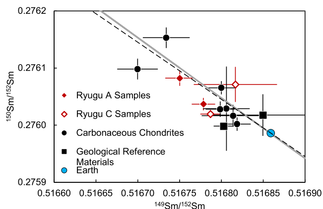
FIGURE 6. ^{150}\text{Sm}/^{152}\text{Sm} versus ^{149}\text{Sm}/^{152}\text{Sm} for the Ryugu “A” (solid red diamonds) and “C” (open red diamonds) samples, carbonaceous chondrites (black circles), and geological reference materials (black squares) measured in this study. The black dashed line is a calculated correlation line resulting from changing one atom of ^{149}\text{Sm} to ^{150}\text{Sm} . The solid gray line indicates the correlation line of lunar samples from Boyet and Carlson (2007). The blue point shows the high-precision Sm isotopic composition of the AMES Sm standard that presumably represents the Sm isotopic composition of the bulk Earth (Carlson et al., 2007). (Color figure can be viewed at wileyonlinelibrary.com )
