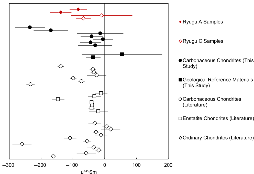
FIGURE 5. The \mu^{149}\text{Sm} compositions of Ryugu “A” (solid red diamonds) and “C” (open red diamonds) samples, carbonaceous chondrites (black circles), and geological reference materials (black squares) from this study and carbonaceous chondrites (white circles; Boyet & Carlson, 2005; Carlson et al., 2007), enstatite chondrites (white squares; Bouvier & Boyet, 2016; Boyet & Carlson, 2005; Carlson et al., 2007; Frossard et al., 2022), and ordinary chondrites (white diamonds; Boyet & Carlson, 2005; Carlson et al., 2007; Frossard et al., 2022) from previous studies. (Color figure can be viewed at wileyonlinelibrary.com )
