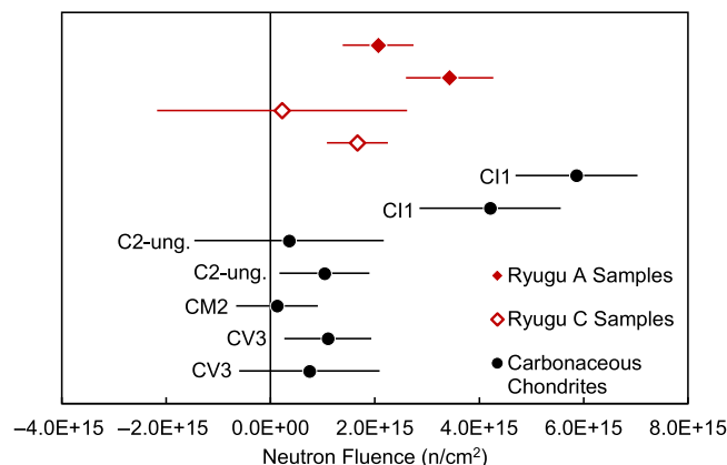
FIGURE 7. Neutron fluence ( \psi ) for the carbonaceous chondrites (black circles) and Ryugu “A” (solid red diamonds) and “C” (open red diamonds) samples measured in this study. (Color figure can be viewed at wileyonlinelibrary.com )
