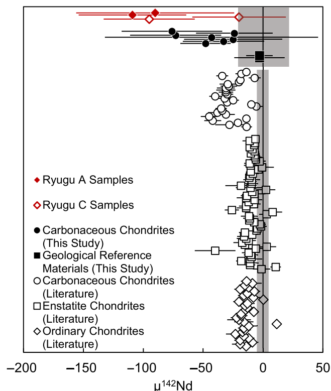
FIGURE 2. The \mu^{142}\text{Nd} compositions of Ryugu “A” (solid red diamonds) and “C” (open red diamonds) samples, carbonaceous chondrites (black circles), and geological reference materials (black squares) from this study and ordinary chondrites (white diamonds), enstatite chondrites (white squares), and carbonaceous chondrites (white circles) from previous studies (Andreasen & Sharma, 2006; Boyet et al., 2018; Bouvier & Boyet, 2016; Boyet & Carlson, 2005; Burkhardt et al., 2016; Carlson et al., 2007; Frossard et al., 2022; Fukai & Yokoyama, 2017, 2019; Gannoun et al., 2011; Johnston et al., 2022; Saji et al., 2020). The data from this study and most previous studies are corrected for ^{146}\text{Sm} decay to an average chondritic ^{147}\text{Sm}/^{144}\text{Nd} = 0.1960 (Bouvier et al., 2008). The gray shaded regions indicate the 2SD of our repeated measurements of the BCR-2 standard ( \pm 21 ppm) and the average 2SD of previous measurements ( \pm 5 ppm). (Color figure can be viewed at wileyonlinelibrary.com )
