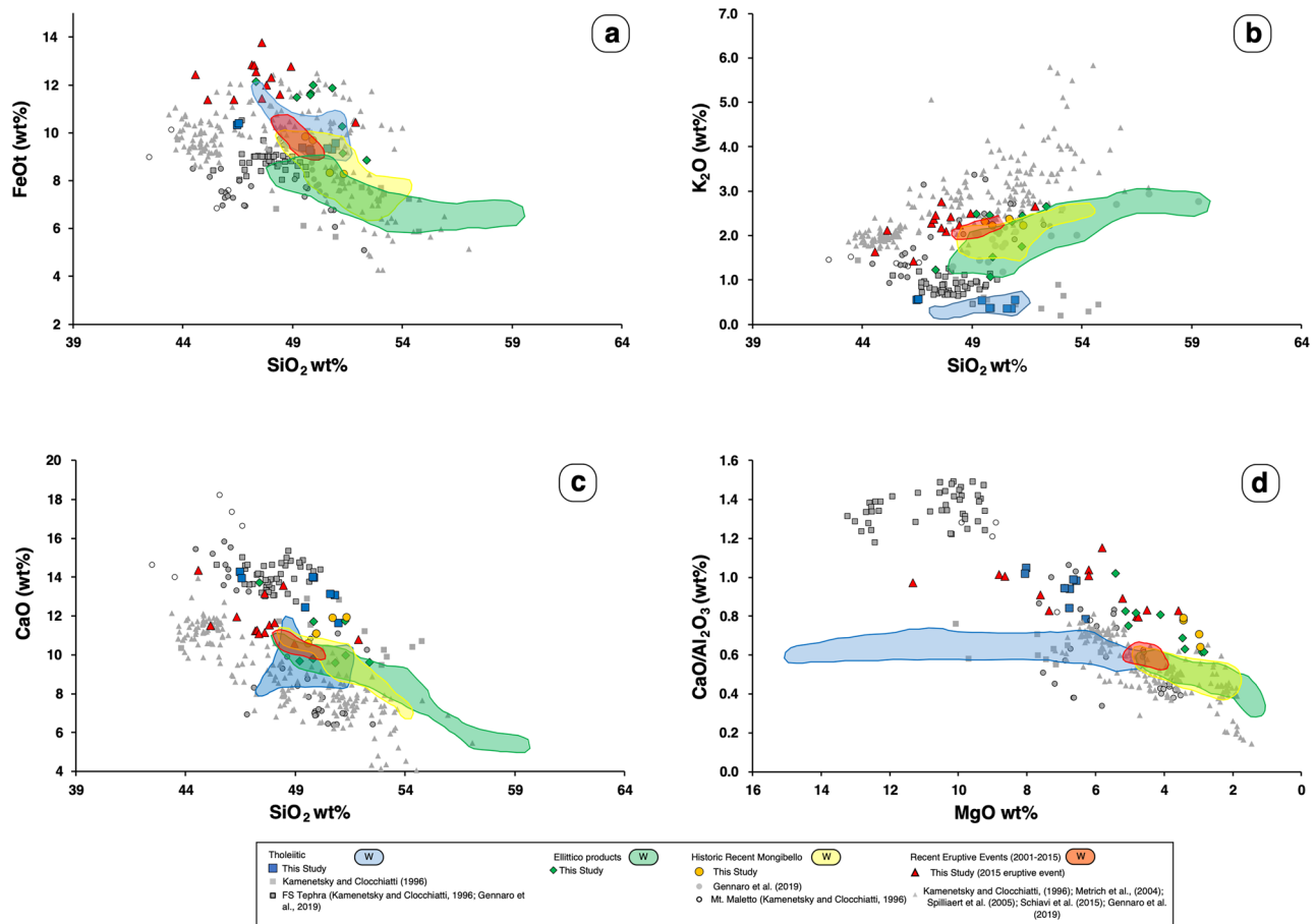
Fig. 4 Harker variation diagrams showing major element composition of studied MIs and bibliographic data: a \text{SiO}_2 vs \text{FeO}_t ; b \text{SiO}_2 vs \text{K}_2\text{O} ; c \text{SiO}_2 vs \text{CaO} and d \text{MgO} vs \text{CaO}/\text{Al}_2\text{O}_3
