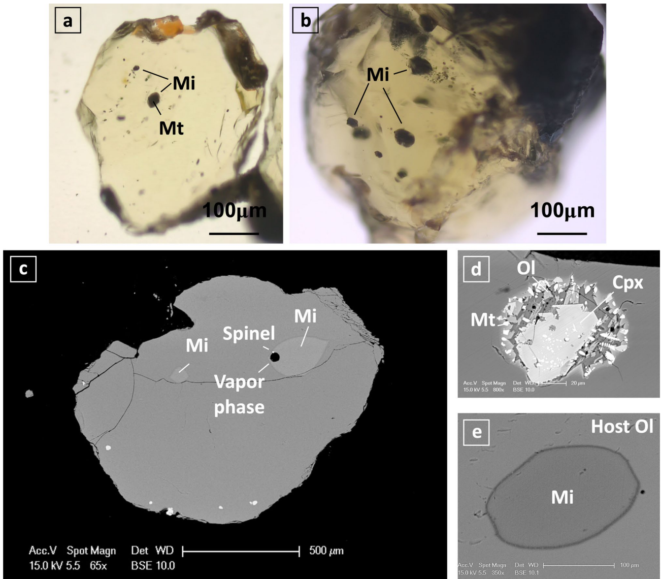
Fig. 1 Microphotographs of studied a MIs hosting olivine crystal before and after HP-HT homogenization experiments. In panels a and b ; transmitted light microphotographs of olivine grains containing several MIs before re-homogenization experiments. c Backscattered SEM images of olivine hosting melt-inclusion after the homogeni-
