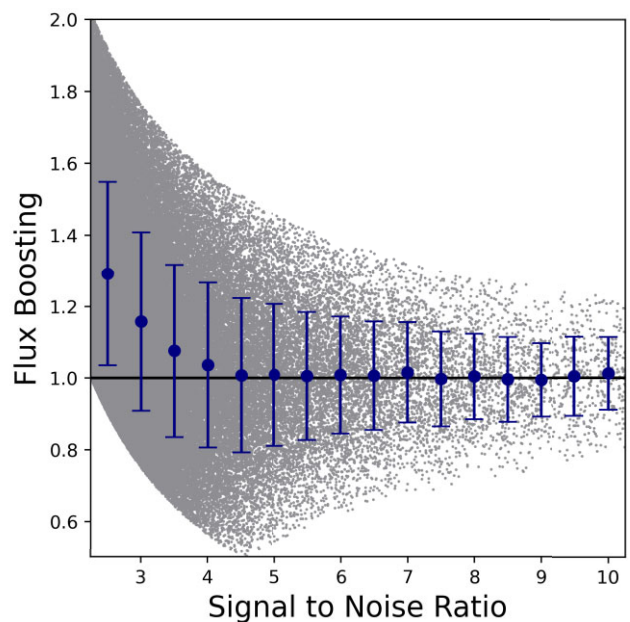
Figure 5. The flux boosting (i.e. the extracted/injected flux ratio) at 850 \mu\text{m} is estimated from the fake injected sources (grey dots), where the detected faint sources likely have fainter fluxes. The blue errorbars indicate the averaged flux boosting within SNR bins with a width of 0.5\sigma . We adjust for the flux boosting for the 850 \mu\text{m} fluxes in Table 2, and include the additional uncertainty to the instrumental uncertainty in quadrature.
