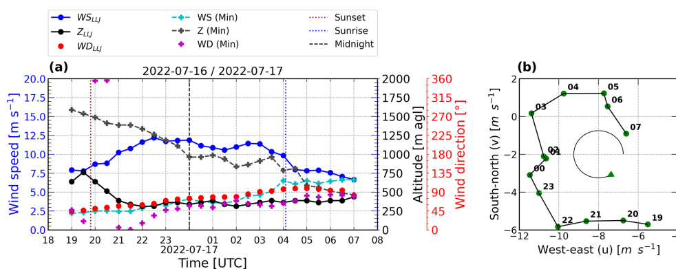
Figure 6. Nocturnal evolution of an individual LLJ event (16–17 July 2022). Panel (a) illustrates the jet characteristics: core wind speed ( WS_{LLJ} ) and the minimum above ( WS_{Min} ), core height ( Z_{LLJ} ) and the height of the minimum above ( Z_{Min} ), and core wind direction ( WD_{LLJ} ) and wind direction of the minimum above ( WD_{Min} ). Panel (b) shows the wind hodograph based on the zonal and meridional components of the wind ( u, v ) at the height of the core of the jet. The green arrow indicates the sense in which the wind is veering during the night (clockwise). Labels indicate the hour from 19:00 on 16 July to 07:00 on 17 July (UTC).
