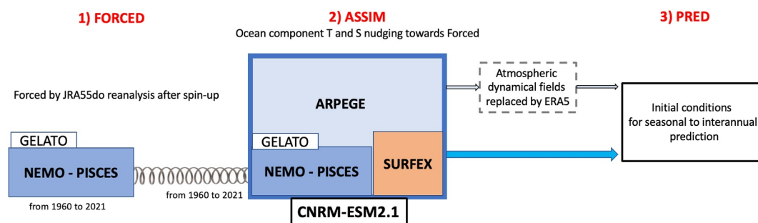
Figure 1. Schematics of the initialization procedure of the C3PS platform. The “spring” connecting the two NEMO-PISCES boxes indicates that the coupled simulation is relaxed to potential temperature and salinity in the forced simulation.
