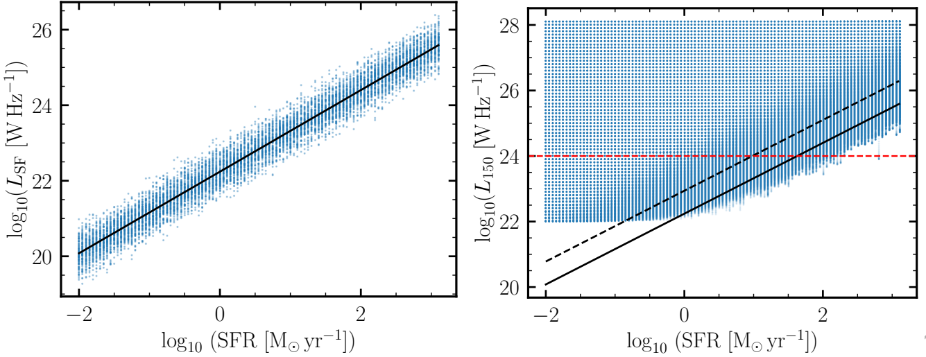
Figure A1. Results of the Monte Carlo simulation to quantify the completeness of the radio-excess AGN selection. Left: The simulated relationship between the 150 MHz radio-luminosity and star-formation rate for star-forming galaxies, with a simulated Gaussian scatter of 0.3 dex. Right: The total 150 MHz radio luminosity for simulated sources, calculated as the sum of the L_{\text{AGN}} and L_{\text{SF}} components (from the left panel), as a function of the star-formation rate (see text). The black solid line in both panels shows the radio luminosity – star-formation rate relation of Best et al. (2023). The dashed black line shows the radio-excess criterion (0.7 dex above the relation) used to identify radio-excess AGN. The red line corresponds to the radio luminosity limit of L_{150\text{MHz}} \geq 10^{24} \text{ W Hz}^{-1} applied for the analysis
