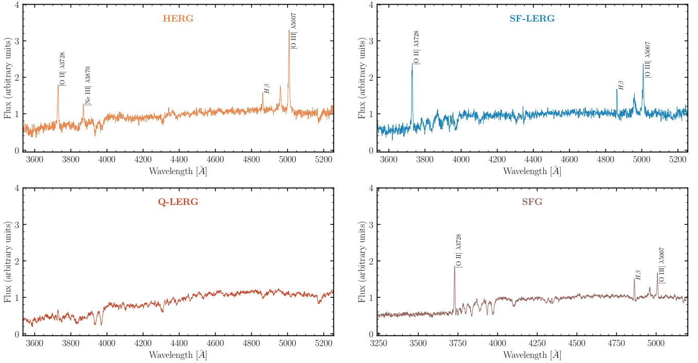
Figure B1. The median stacked spectra for HERGs, SF-LERGs, Q-LERGs, and SFGs across 0.5 < z \leq 1 . The individual spectra, derived from the DESI EDR (DESI Collaboration et al. 2023), are shifted to the rest-frame, normalised and resampled onto a common wavelength grid before computing a median stacked spectrum. The Q-LERG stack shows Ca H and K absorption features, indicative of an old stellar population, with no signs of emission lines associated with either star-formation or AGN activity. The HERG stack show strong detection of high-excitation emission lines, such as [Ne III] and [O III], and an [O III]/ h\beta ratio associated with the presence of AGN activity.
