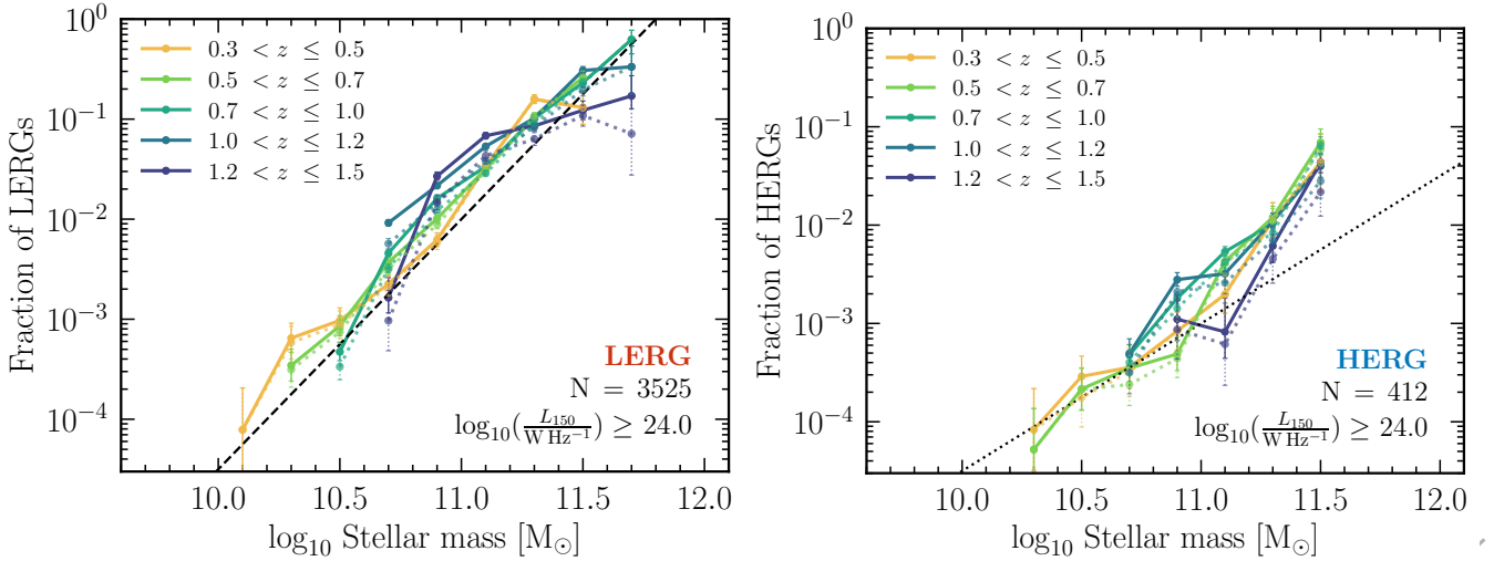
Figure 1. The fraction of all galaxies that host a LERG (left) or a HERG (right) as a function of stellar mass across 0.3 < z \leq 1.5 for a radio luminosity limit of L_{150\text{MHz}} \geq 10^{24} \text{ W Hz}^{-1} . The numbers of LERGs and HERGs satisfying the radio luminosity limit over this redshift range are also listed in each panel. The solid and dotted lines show the fractions obtained with and without the radio-luminosity – SFR completeness corrections, respectively (see text and Appendix A); these corrections have a small effect for the overall populations. The black dashed line in the left panel represents the steep stellar mass relation ( \propto M_*^{2.5} , normalised to 0.01 at M = 10^{11} M_\odot ) found for LERGs in the local Universe (Best et al. 2005a; Janssen et al. 2012). The black dotted line in the right panel corresponds to the shallow mass dependence ( \propto M_*^{1.5} , normalised to 0.001 at M = 10^{11} M_\odot ), similar to that found for HERGs in the local Universe (Janssen et al. 2012). The LERGs show the same steep relation as observed in the local Universe all the way out to z \sim 1.5 . The HERG fraction at low masses follow a shallower relation at M < 10^{11} M_\odot , but show a steeper than expected relation (based on higher frequency local Universe studies) at higher masses.
