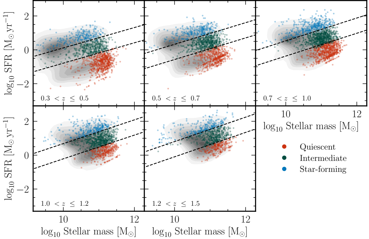
Figure 3. The location of LERGs on the SFR- M_* plane in five redshift bins across 0.3 < z \leq 1.5 . The LERG sample has been split into the subset that are hosted by quiescent (red), intermediate (green), and star-forming (blue) galaxies, defined based on the evolving main-sequence (see Sec. 4). The diagonal dashed lines show the division lines used to select the three populations. The shaded contours show the distribution of the underlying MIR flux-selected parent sample along the SFR- M_* plane.
