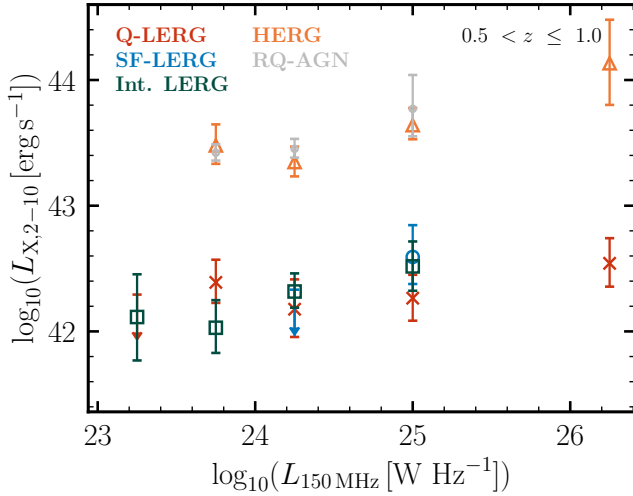
Figure B2. The median stacked 2-10 keV rest-frame X-ray luminosities as a function of radio luminosity for LERGs hosted by different galaxy types, HERGs, and RQ-AGN across 0.5 < z \leq 1.0 . The stacked X-ray luminosities represent the median X-ray luminosities based on bootstrap resampling, which are corrected for the contribution from XRBs. The uncertainties are computed using the corresponding bootstrap method. At a given radio luminosity, the LERGs, regardless of their host galaxy star-formation activity, show over an order of magnitude lower X-ray luminosities than the HERGs or RQ-AGN.
