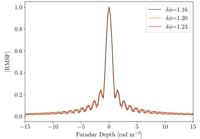
Fig. 3. RMSF functions of observations with different frequency ranges (see Table 1). The difference between the functions is marginal.
