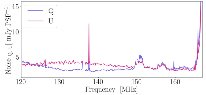
Fig. 2. Noise in Stokes Q and U for a randomly chosen frequency cube that was not corrected for the primary beam.
