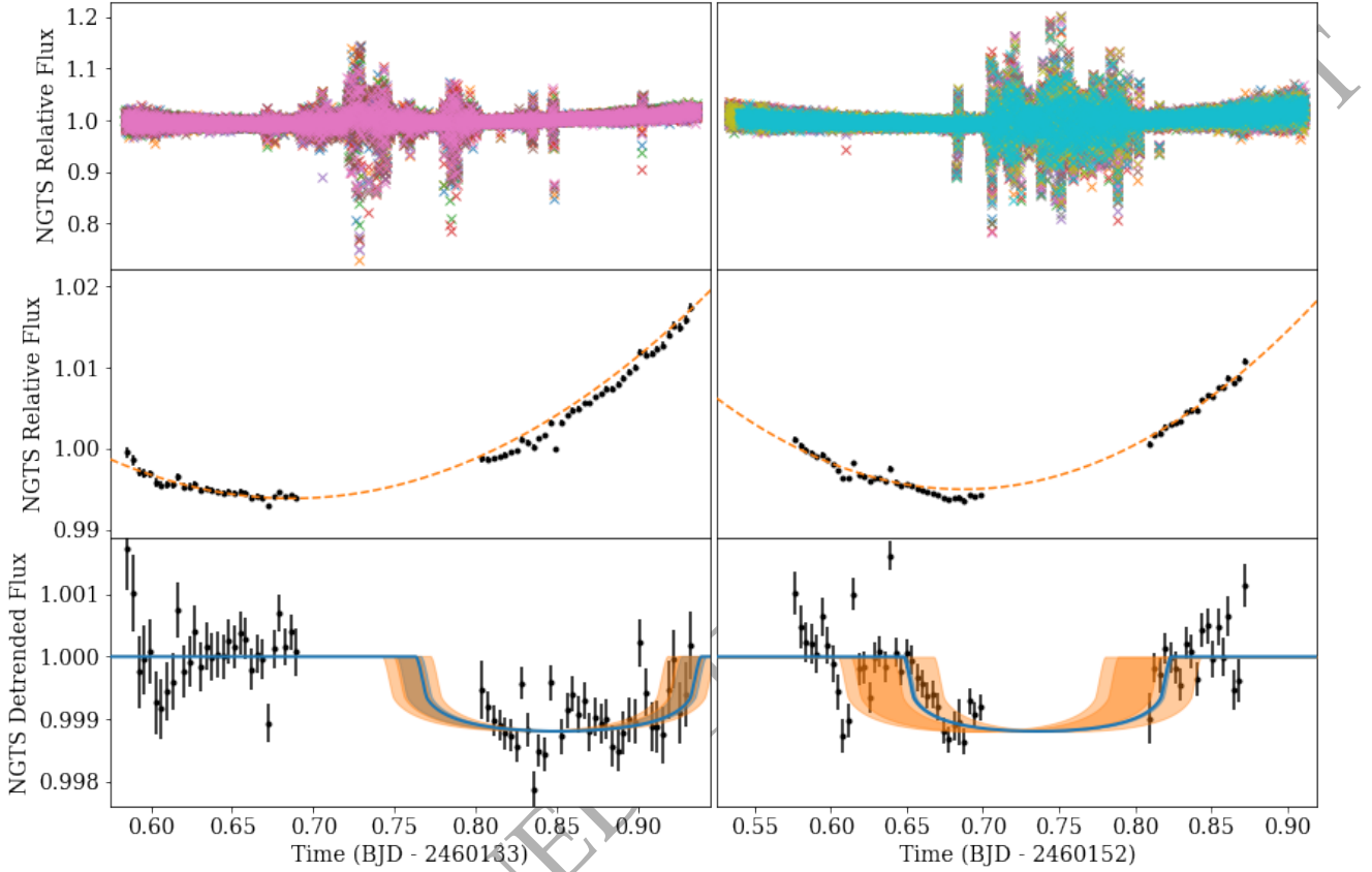
Figure C1. NGTS photometric observations of the AU Mic transits. The left and right columns show the first and second visits, respectively. The top row shows the full observations for all telescopes used, with data from each individual telescope plotted using a different colour. The middle row shows the data with the cloud-affected portion removed, and with the data from all telescopes binned together at a timescale of 5 minutes (the binning is performed for visualisation purposes only, the analysis was performed on the unbinned data). The orange dashed line in the middle row shows the best-fit polynomial component to the NGTS data. The bottom row shows the data after subtracting the polynomial component. The blue line shows the best fit model from the NGTS analysis with the blue shaded region showing the 68% credible interval. The dark and light orange shaded regions give the 67.3% and 95% credible intervals respectively from the CHEOPS-ESPRESSO joint analysis.
