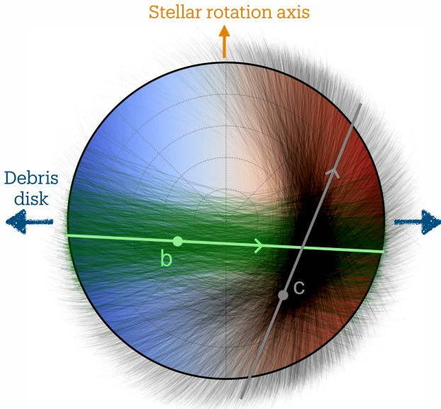
Figure 7. Schematic representation of the spin-orbit alignment of planets b and c within the AU Mic system. The stellar disk is colour-coded to represent local RVs, which vary as the star rotates, transitioning from blue-shifted on the left to red-shifted on the right. The bold green and grey lines represent the inferred orbits for planet b from Palle et al. (2020) and planet c from this work, with arrows indicating the directions of motion for the planets. Thin green and grey lines represent 50,000 randomly selected samples for the orbit of planets b and c, respectively. For the orbit of planet c, the transparency of the thin grey lines scales as the weight of each sample in the nested sampling. The orange arrow marks the axis of stellar rotation. The dark blue arrow marks the orientation of the debris disk.
