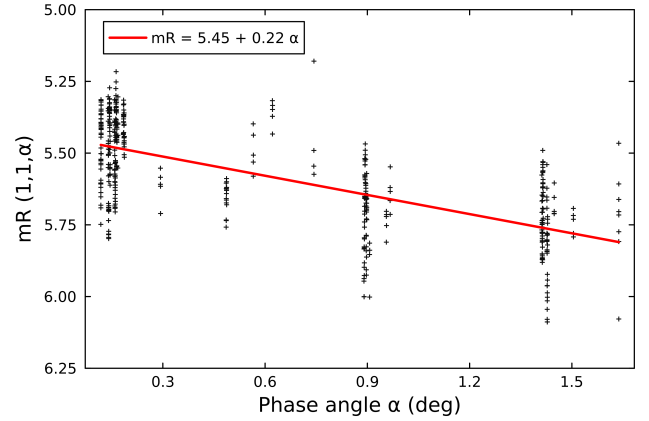
Fig. 4. Reduced magnitude m_R(1, 1, \alpha) vs. the phase angle, \alpha . In total, 431 observations were obtained with the 2 m LT, with the 1.5 m telescope at Sierra Nevada Observatory, and with the 1.23 m telescope at Calar Alto Observatory were used. The brightness variation cluster is due to the rotation of 2003 UY 117 .
