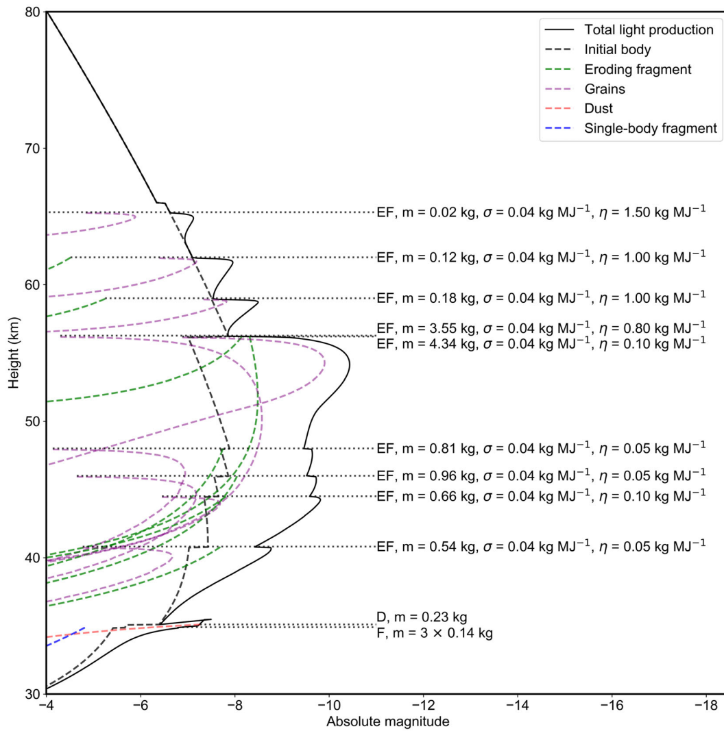
FIGURE 7. Details of individual fragmentation events. The fragmentation points, the type of fragmentation, total fragment mass, fragment ablation, and erosion coefficients are shown. (Color figure can be viewed at wileyonlinelibrary.com )
