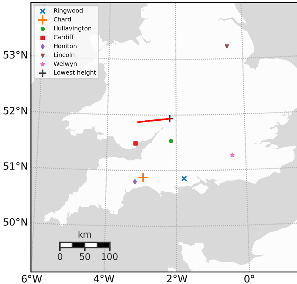
FIGURE 2. The Winchcombe fireball trajectory (red line) and locations of cameras used for astrometric measurements. (Color figure can be viewed at wileyonlinelibrary.com )
