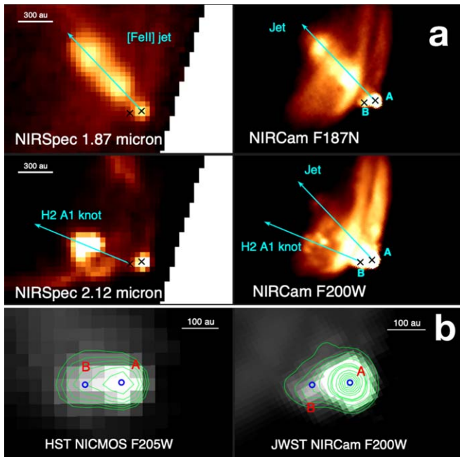
Figure 6. (a) NIRSpect images of line+continuum emission at 1.87 and 2.12 \mu\text{m} (left) are compared with archival NIRCam images in the F187N and F200W filters (right). The NIRCam images (spatial resolution 31 \text{ mas pixel}^{-1} ) reveal a secondary source (B) located at about 0''.23 from the primary (A), i.e., about the position where Reipurth et al. (2000) reported the detection of a companion. The arrows indicate the direction of the jet axis driven by source A, and the H_2 A1 arc-shaped knot apparently pointing toward source B. (b) Comparison of a HST image in the F205W filter of the HH46 IRS binary taken in 1998 with the NIRCcam F200W image taken in 2023. Blue circles in both images indicate the position of sources A and B in the HST image. Source B appears to have rotated around source A by about 13^\circ counterclockwise.
